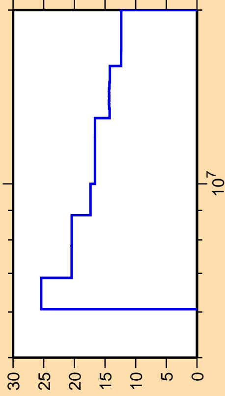
\Delta\sigma/\sigma vs. E for ^{239}\text{Cm}(n,f)
