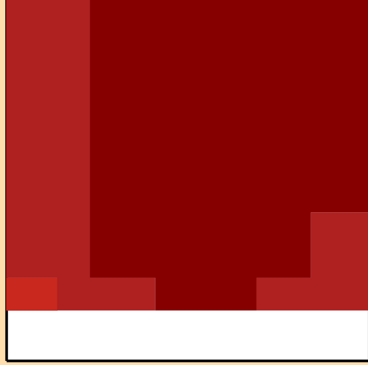
\Delta\sigma/\sigma vs. E for ^{239}\text{Cm}(n,\text{tot.})
