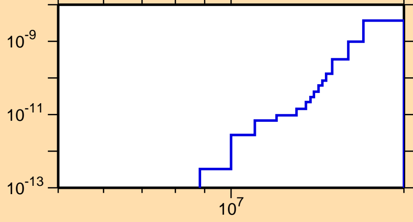
\sigma vs. E for ^{239}\text{Cm}(n,2n\alpha)
