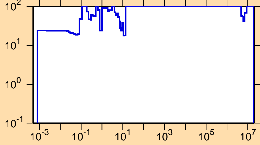
\Delta\sigma/\sigma vs. E for ^{239}\text{Cm}(n,\gamma)
