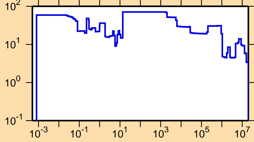
\Delta\sigma/\sigma vs. E for ^{239}\text{Cm}(n,\text{tot.})
