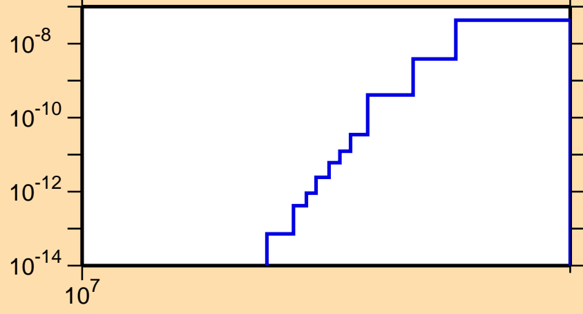
\sigma vs. E for ^{239}\text{Cm}(n,nd)
