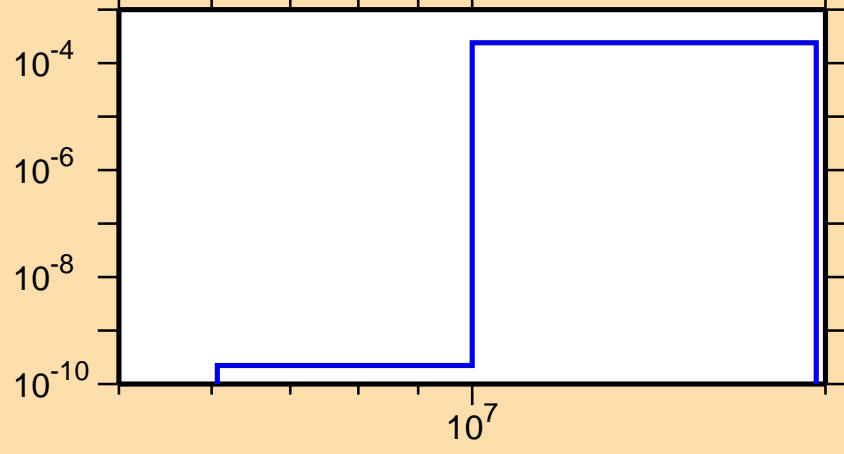
\sigma vs. E for ^{239}\text{Cm}(n,d)
