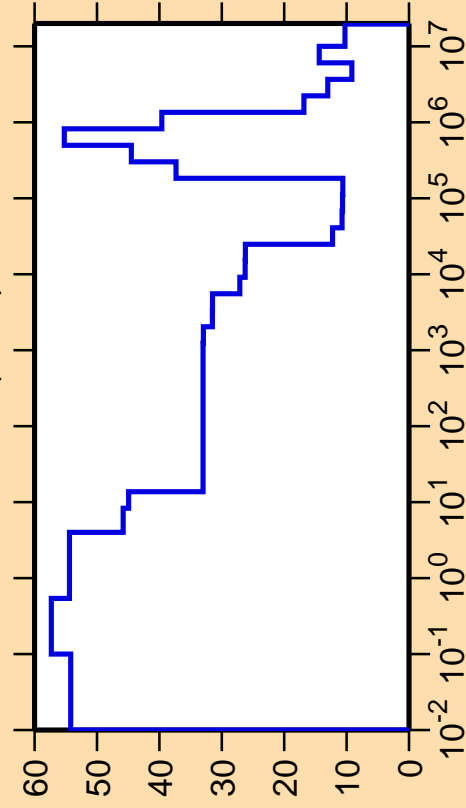
\Delta\sigma/\sigma vs. E for ^{239}\text{Cm}(n,\text{el.})
