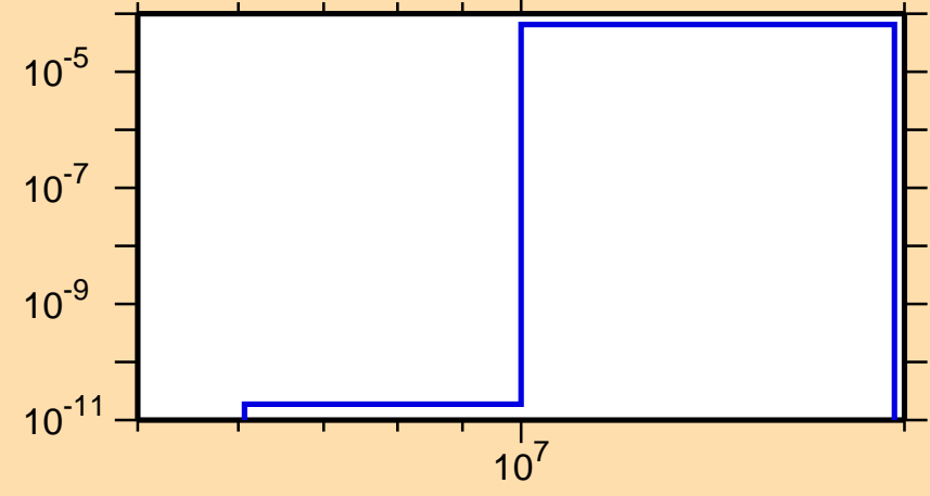
\sigma vs. E for ^{239}\text{Cm}(n,t)
