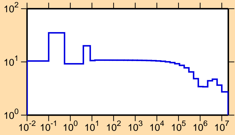
\sigma vs. E for ^{239}\text{Cm}(n,\text{el.})
