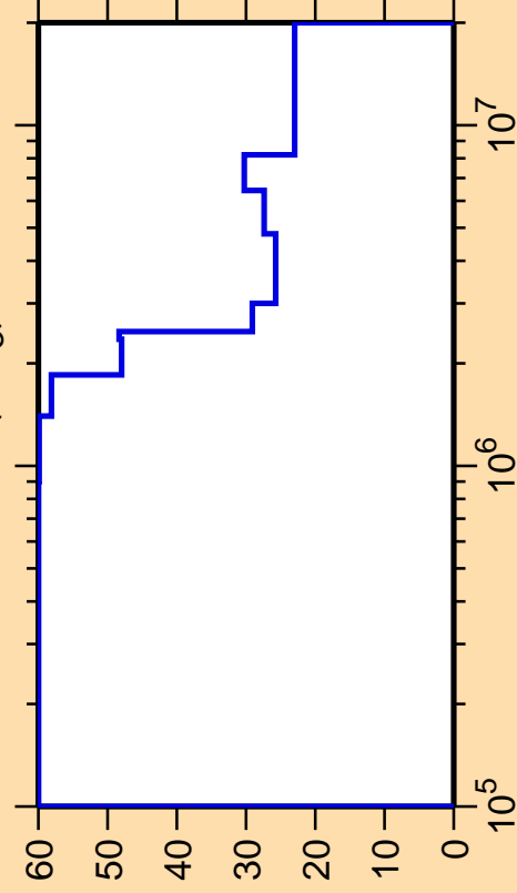
\Delta\sigma/\sigma vs. E for ^{239}\text{Cm}(n,n_3)
