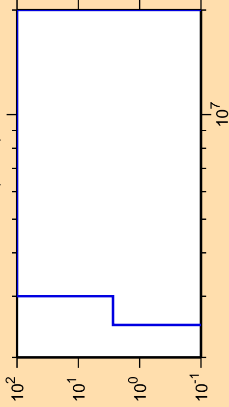
\Delta\sigma/\sigma vs. E for ^{239}\text{Cm}(n,n\alpha)
