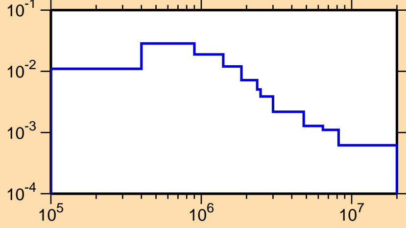
\sigma vs. E for ^{239}\text{Cm}(n,n_3)
