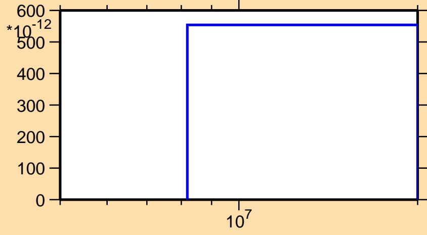
\sigma vs. E for ^{239}\text{Cm}(n,\text{nd})
