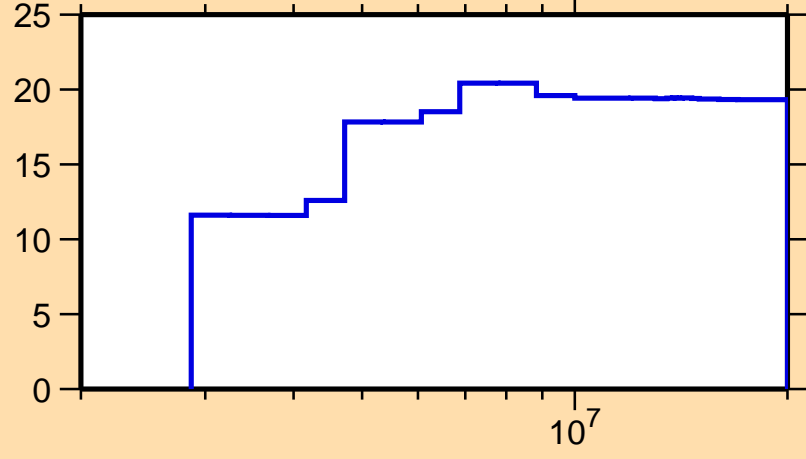
\Delta\sigma/\sigma vs. E for ^{240}\text{Cm}(n,n\text{onel.})
