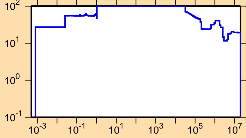
\Delta\sigma/\sigma vs. E for ^{240}\text{Cm}(n,\text{nonel.})
