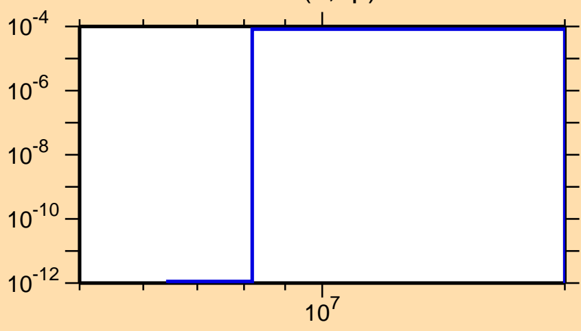
\sigma vs. E for ^{240}\text{Cm}(n,np)
