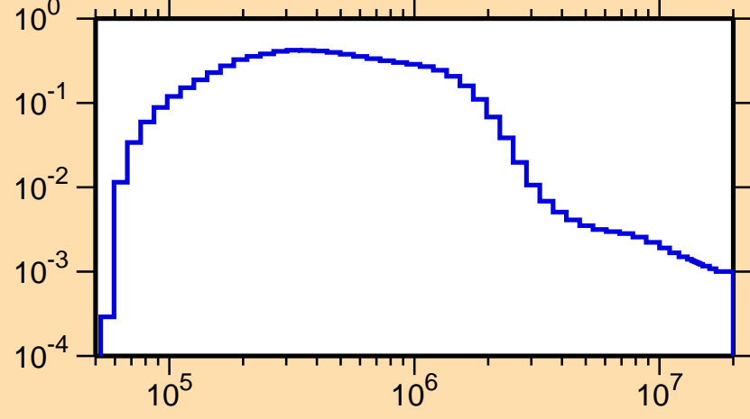
\sigma vs. E for ^{241}\text{Cm}(n,n_2)
