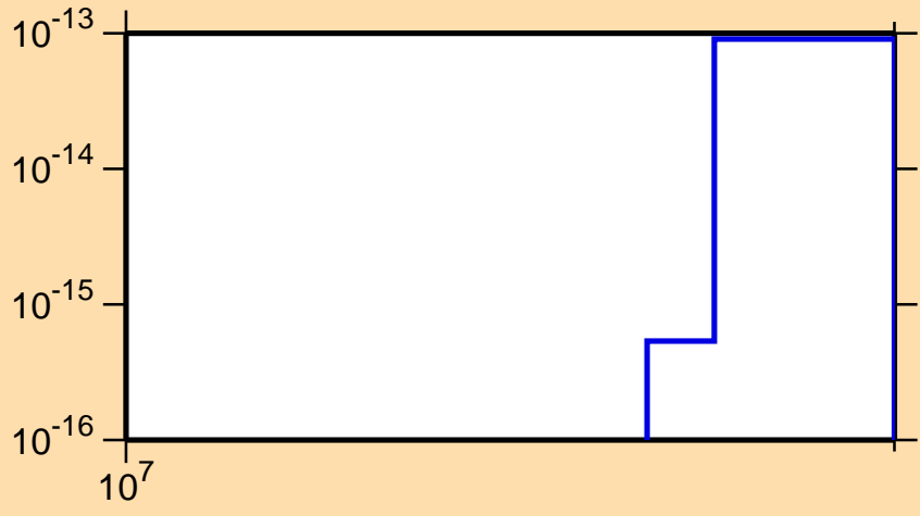
\sigma vs. E for ^{241}\text{Cm} (mt 34)
