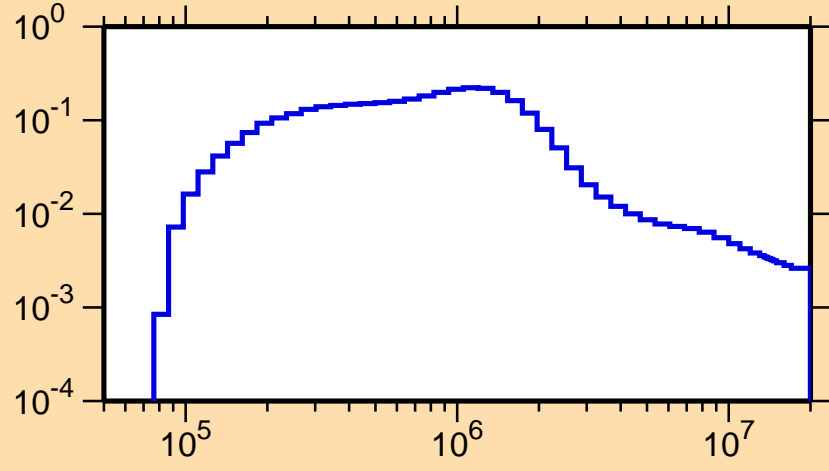
\sigma vs. E for ^{241}\text{Cm}(n,n_3)
