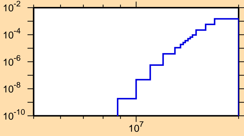
\sigma vs. E for ^{241}\text{Cm}(n,np)
