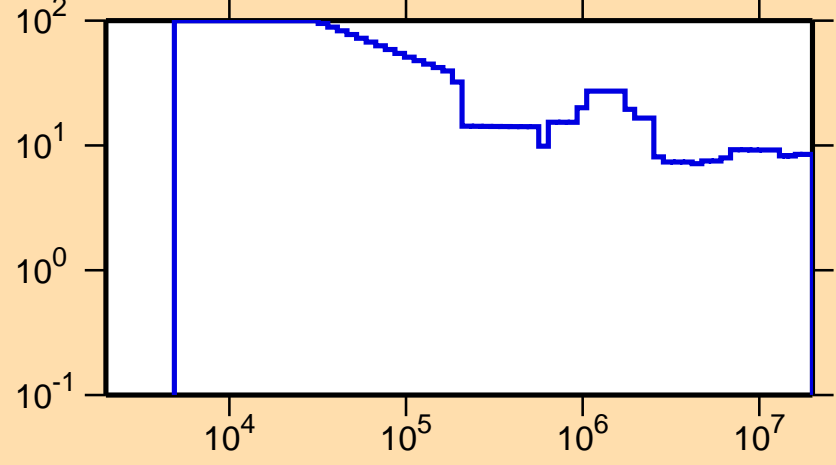
\Delta\sigma/\sigma vs. E for ^{241}\text{Cm}(n,\text{nonel.})
