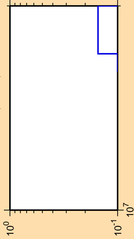
\Delta\sigma/\sigma vs. E for ^{241}\text{Cm} (mt 34)
