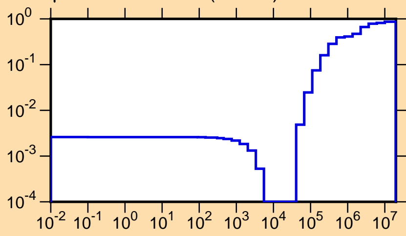
\mu vs. E for ^{241}\text{Cm}(\text{mt251})
