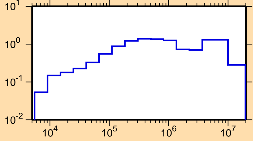
\sigma vs. E for ^{241}\text{Cm}(n,\text{inel.})
