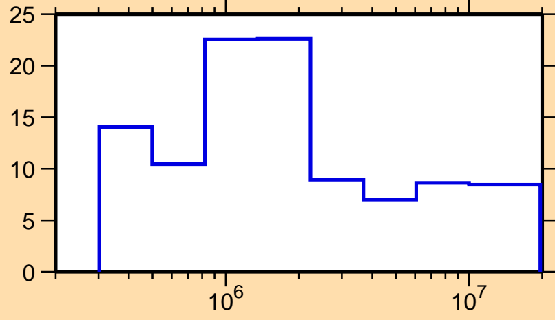
\Delta\sigma/\sigma vs. E for ^{241}\text{Cm}(n,n\text{onel.})
