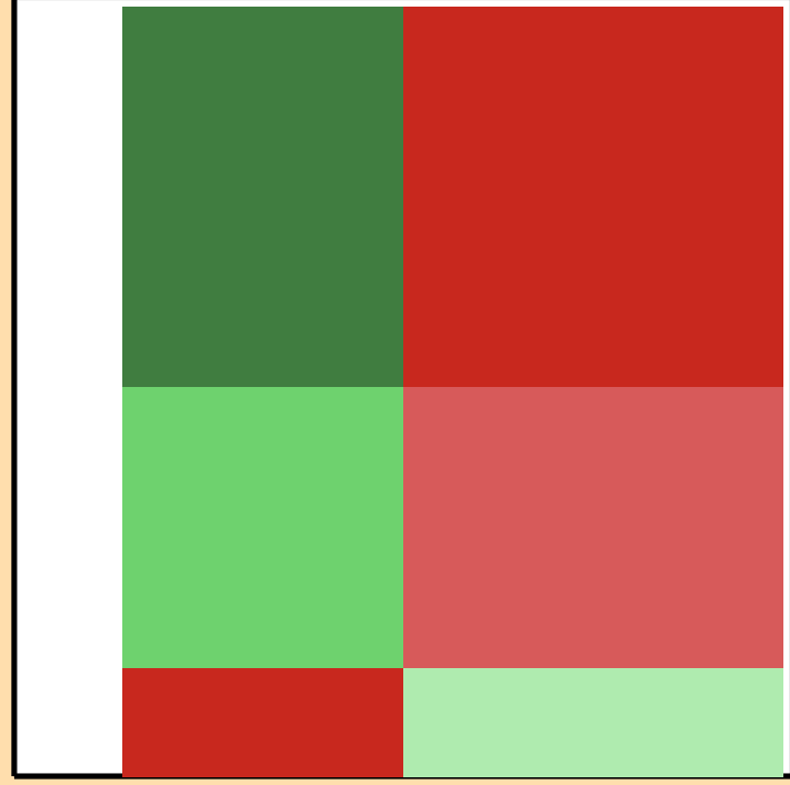
\Delta\sigma/\sigma vs. E for ^{241}\text{Cm}(n,2n)
