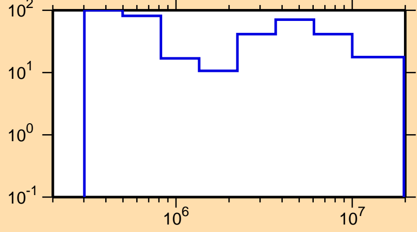
\Delta\sigma/\sigma vs. E for ^{241}\text{Cm}(n,f)
