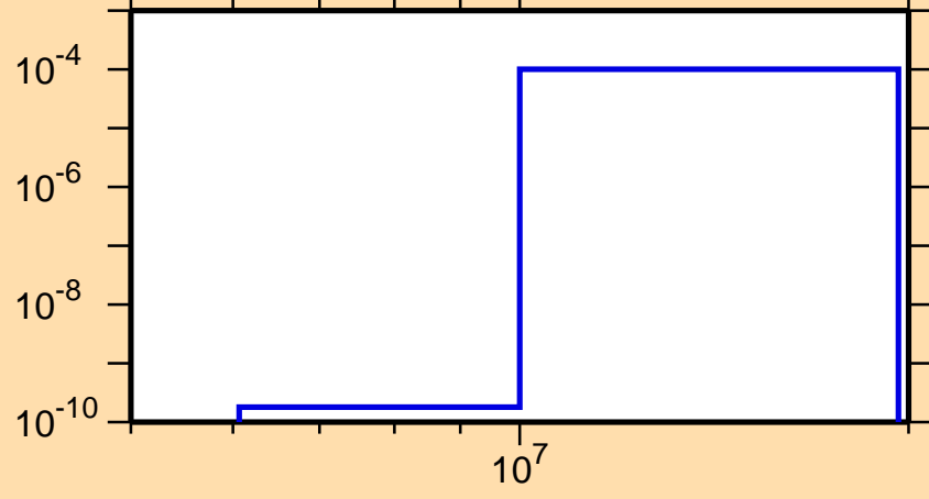
\sigma vs. E for ^{241}\text{Cm}(n,np)
