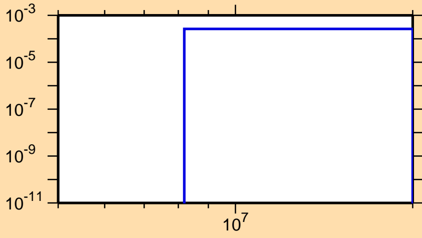
\sigma vs. E for ^{241}\text{Cm}(n,d)
