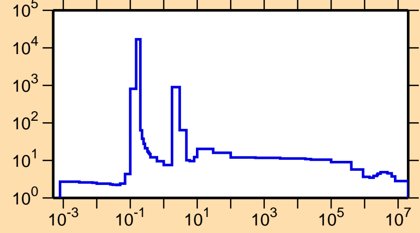
\sigma vs. E for ^{241}\text{Cm}(n,\text{el.})
