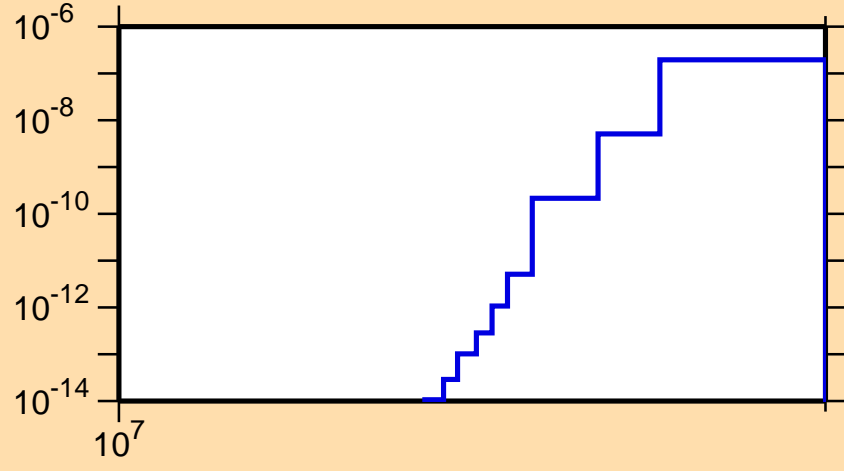
\sigma vs. E for ^{242}\text{Cm}(n,nt)
