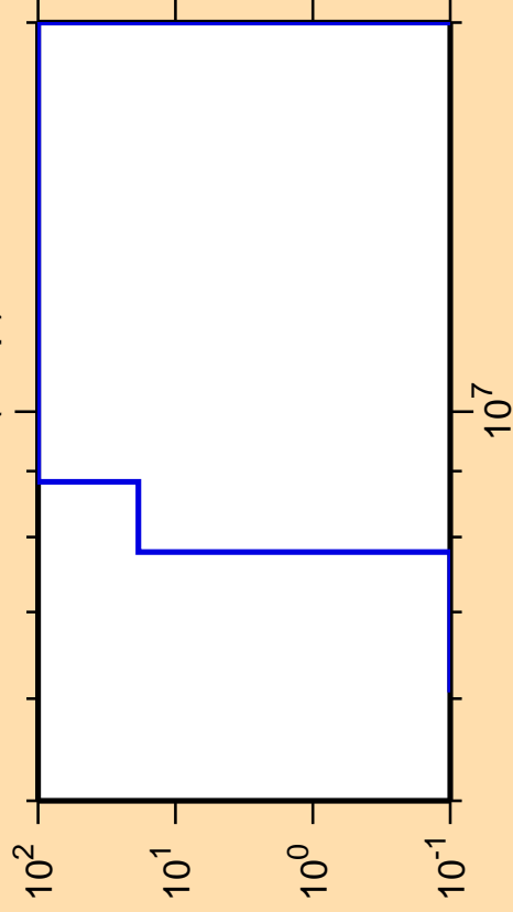
\Delta\sigma/\sigma vs. E for ^{242}\text{Cm}(n,np)
