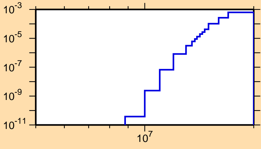
\sigma vs. E for ^{242}\text{Cm}(n,t)
