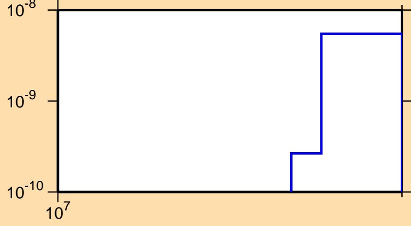
\sigma vs. E for ^{242}\text{Cm}(n,3n\alpha)
