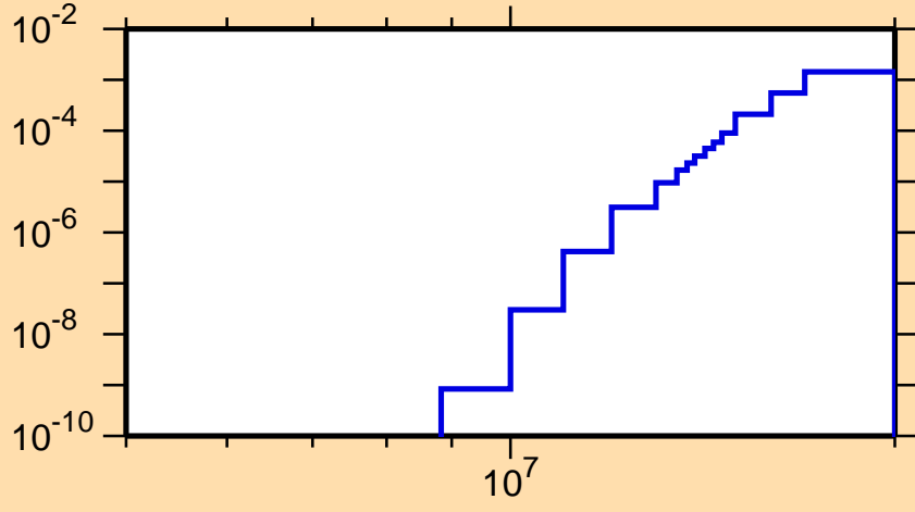
\sigma vs. E for ^{242}\text{Cm}(n,np)
