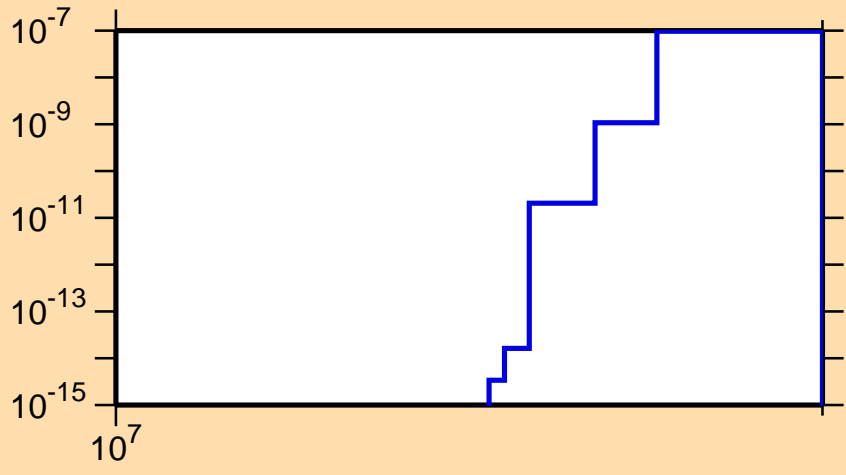
\sigma vs. E for ^{242}\text{Cm}(n,2np)
