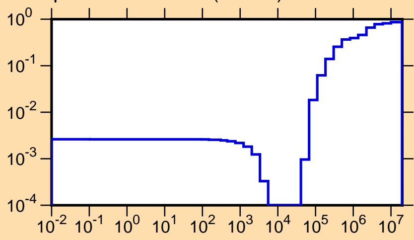
\mu vs. E for ^{242}\text{Cm}(\text{mt251})
