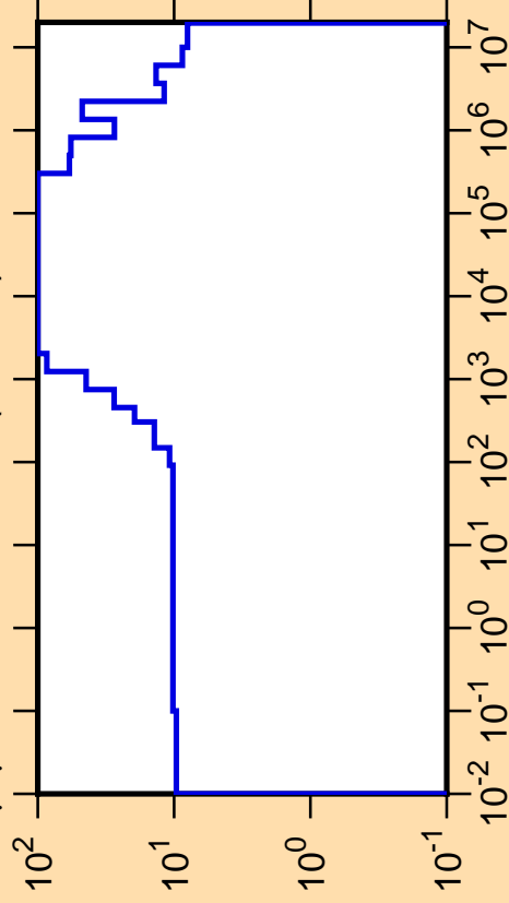
\Delta\mu/\mu vs. E for ^{242}\text{Cm}(\text{mt251})
