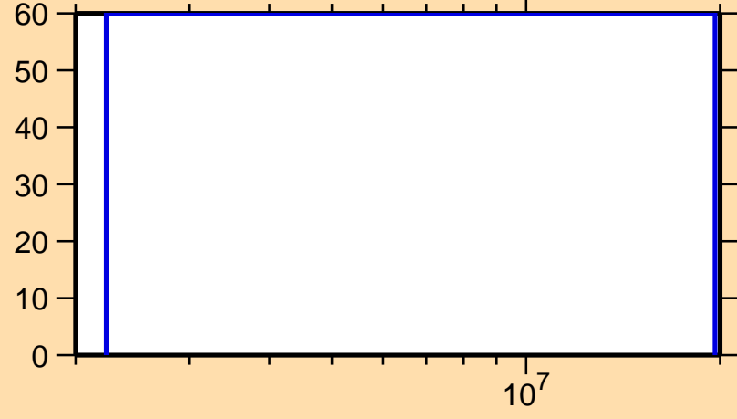
\Delta\sigma/\sigma vs. E for ^{242}\text{Cm}(n,ncont.)
