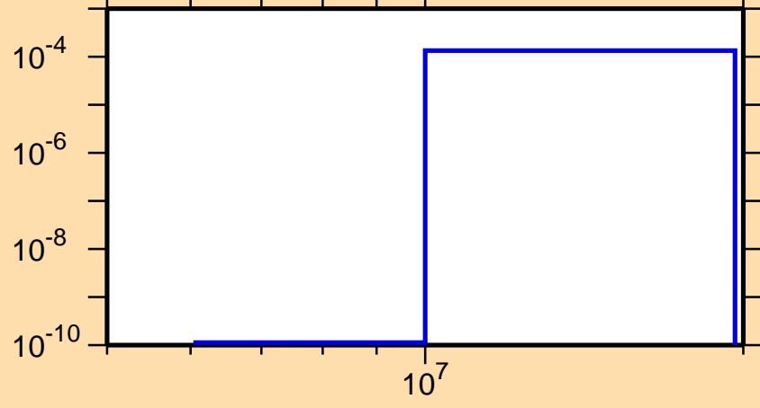
\sigma vs. E for ^{242}\text{Cm}(n,d)
