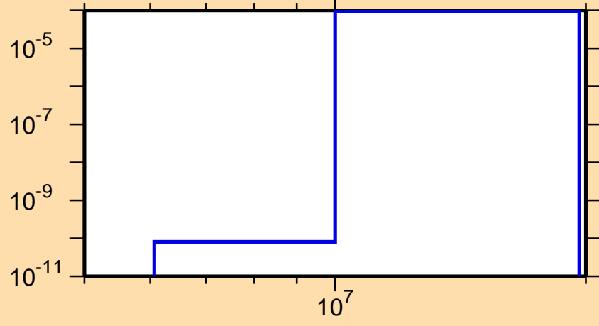
\sigma vs. E for ^{242}\text{Cm}(n,np)
