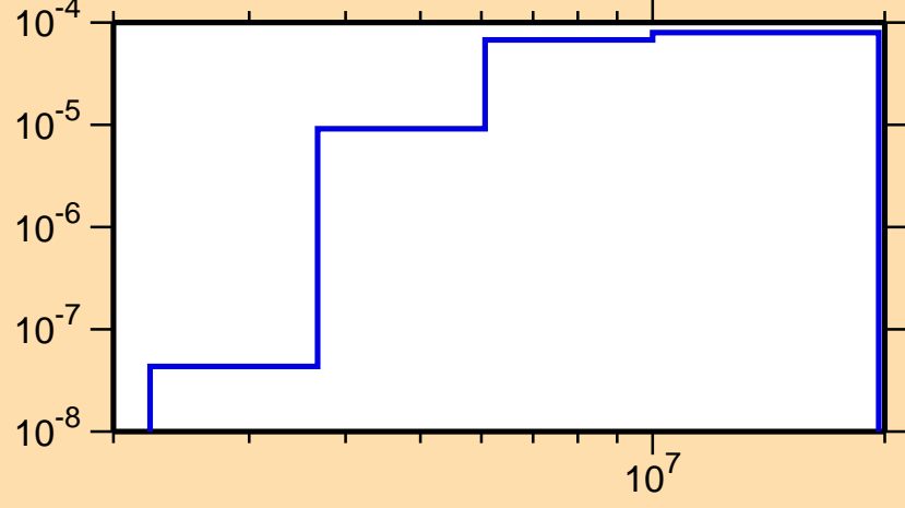
\sigma vs. E for ^{242}\text{Cm}(n,n\alpha)
