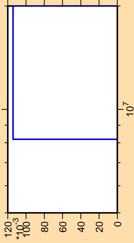
\Delta\sigma/\sigma vs. E for ^{242}\text{Cm}(n,p\alpha)
