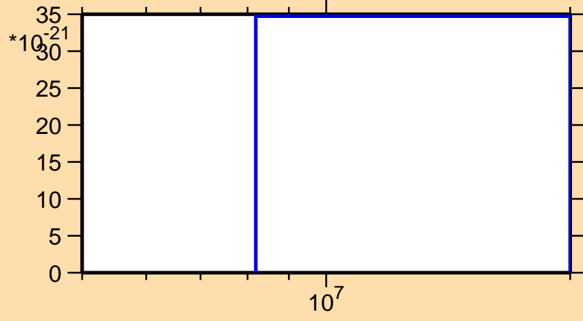
\sigma vs. E for ^{242}\text{Cm} (mt 42)
