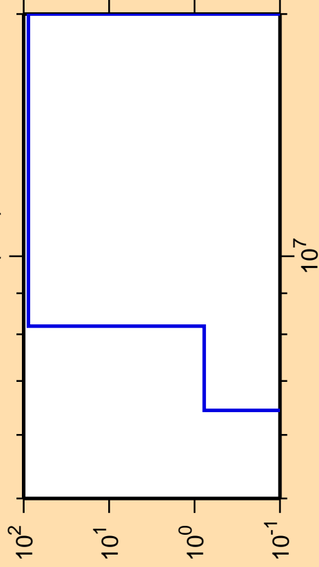
\Delta\sigma/\sigma vs. E for ^{242}\text{Cm}(n,d)
