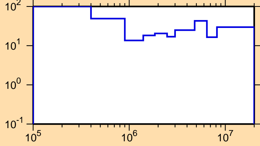
\Delta\sigma/\sigma vs. E for ^{242}\text{Cm}(n,f)
