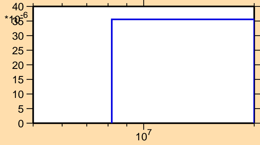
\sigma vs. E for ^{242}\text{Cm}(n,t)
