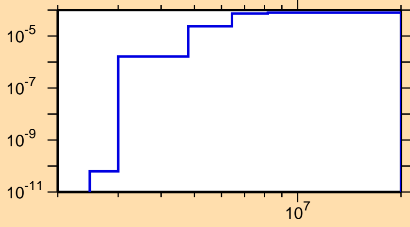
\sigma vs. E for ^{242}\text{Cm}(n,n\alpha)
