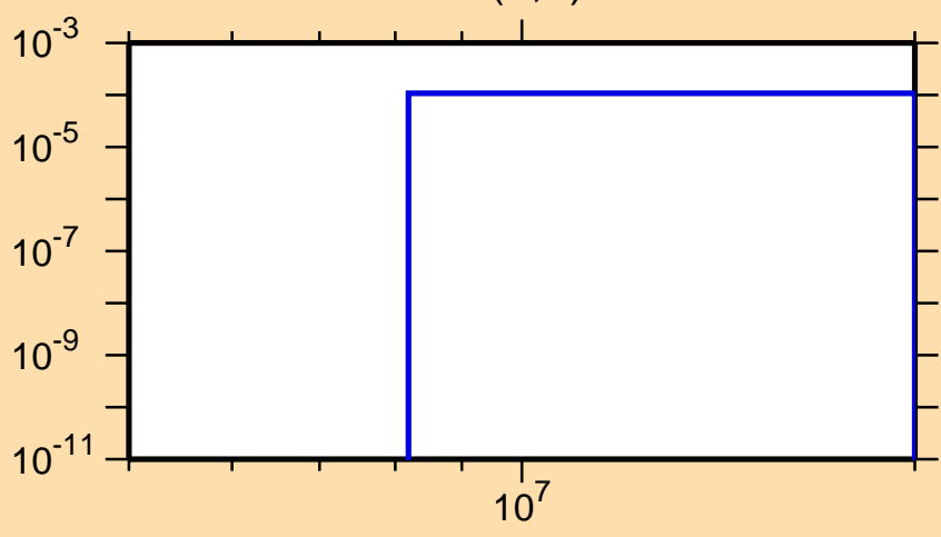
\sigma vs. E for ^{242}\text{Cm}(n,d)
