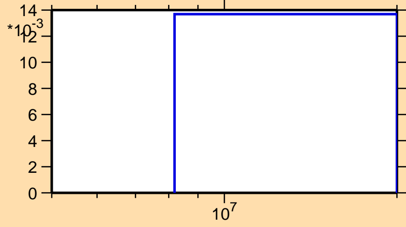
\sigma vs. E for ^{242}\text{Cm}(n,2n\alpha)
