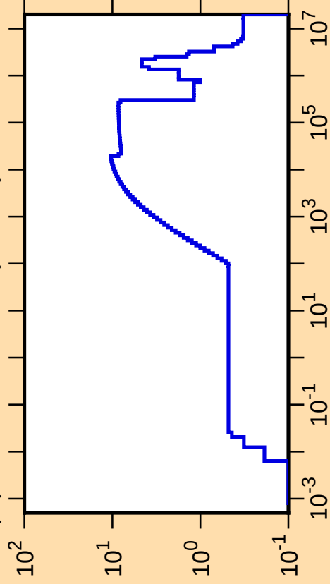
\Delta\mu/\mu vs. E for ^{243}\text{Cm}(\text{mt251})
