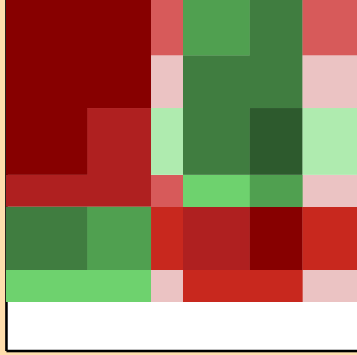
\Delta\sigma/\sigma vs. E for ^{243}\text{Cm}(n,\text{tot.})
