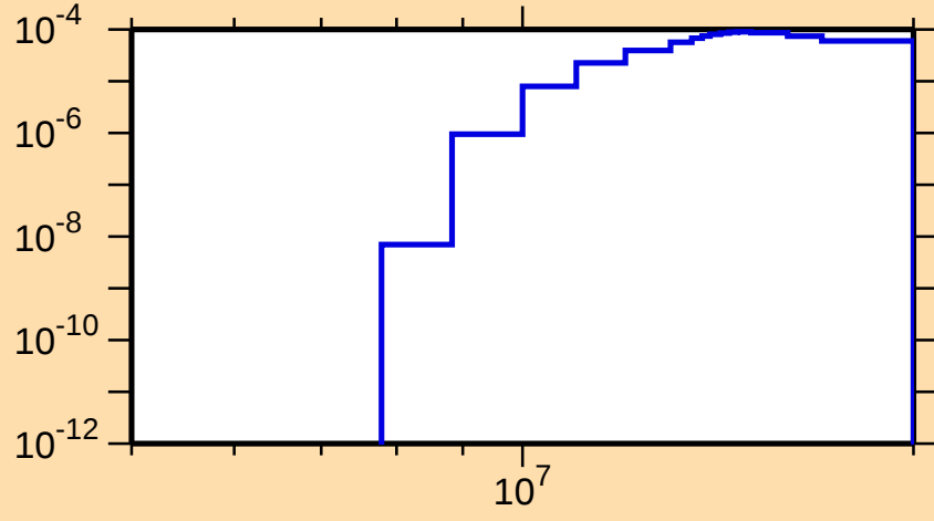
\sigma vs. E for ^{243}\text{Cm}(n,2n\alpha)
