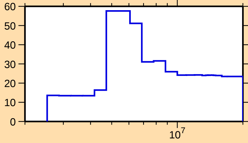
\Delta\sigma/\sigma vs. E for ^{243}\text{Cm}(n,ncont.)
