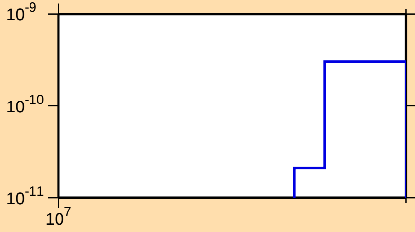
\sigma vs. E for ^{243}\text{Cm}(n,\text{He3})
