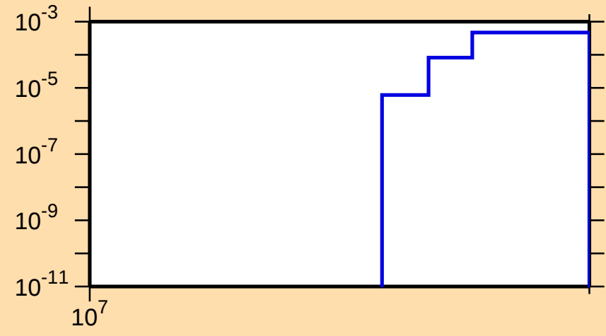
\sigma vs. E for ^{243}\text{Cm}(n,3n\alpha)
