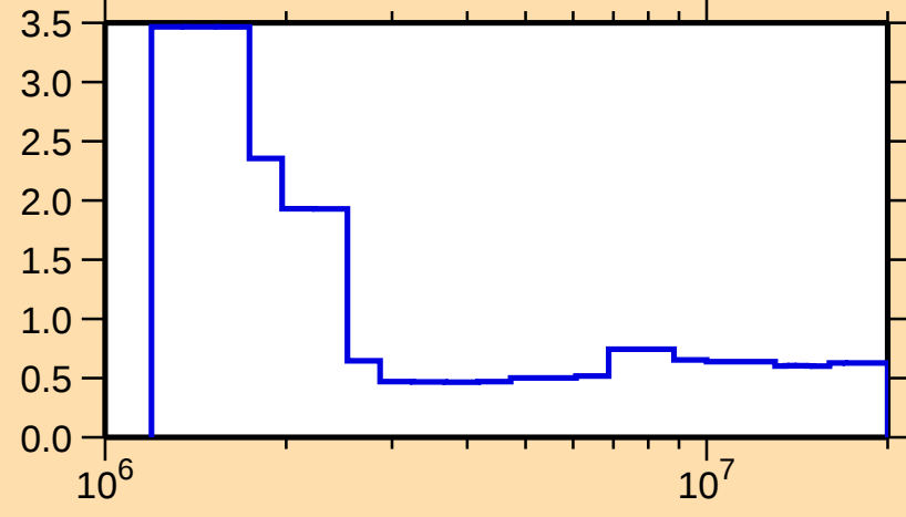
\Delta\sigma/\sigma vs. E for ^{243}\text{Cm}(n,n\text{oncl.})
