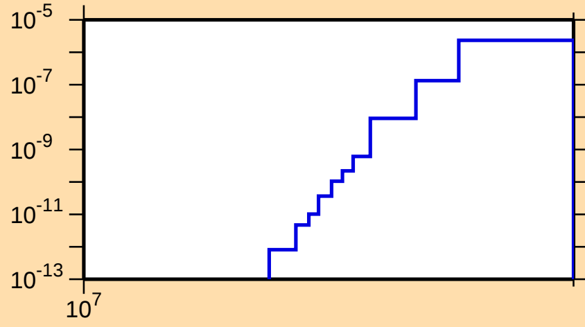
\sigma vs. E for ^{243}\text{Cm}(n,\text{nd})
