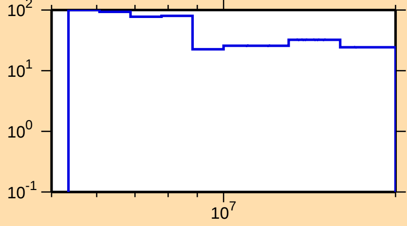
\Delta\sigma/\sigma vs. E for ^{243}\text{Cm}(n,2n)
