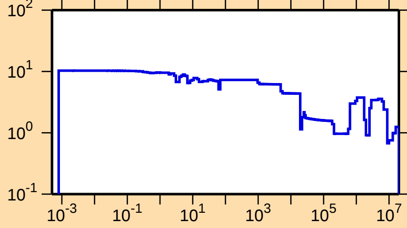
\Delta\sigma/\sigma vs. E for ^{243}\text{Cm}(n,el.)
