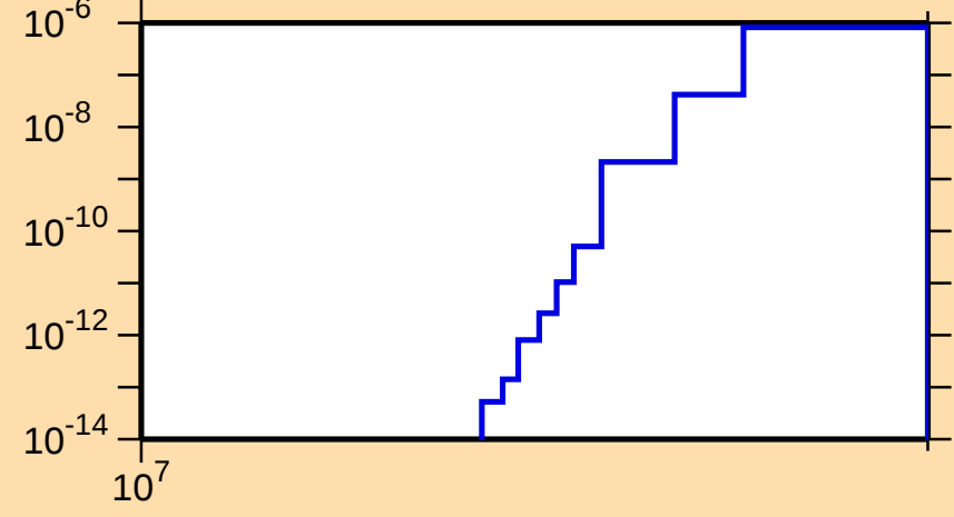
\sigma vs. E for ^{243}\text{Cm}(n,2np)
