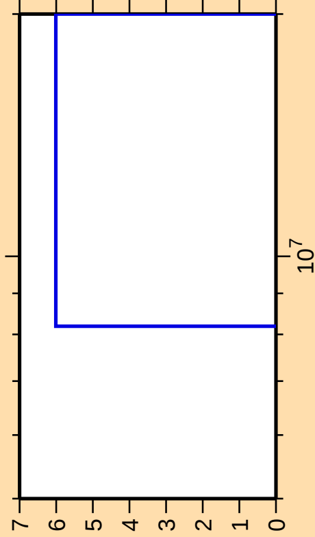
\Delta\sigma/\sigma vs. E for ^{243}\text{Cm}(n,t)
