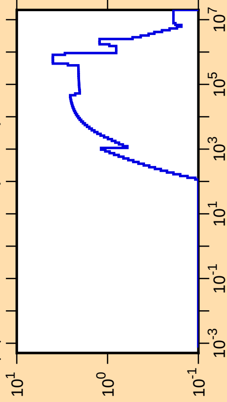
\Delta\mu/\mu vs. E for ^{244}\text{Cm}(\text{mt251})
