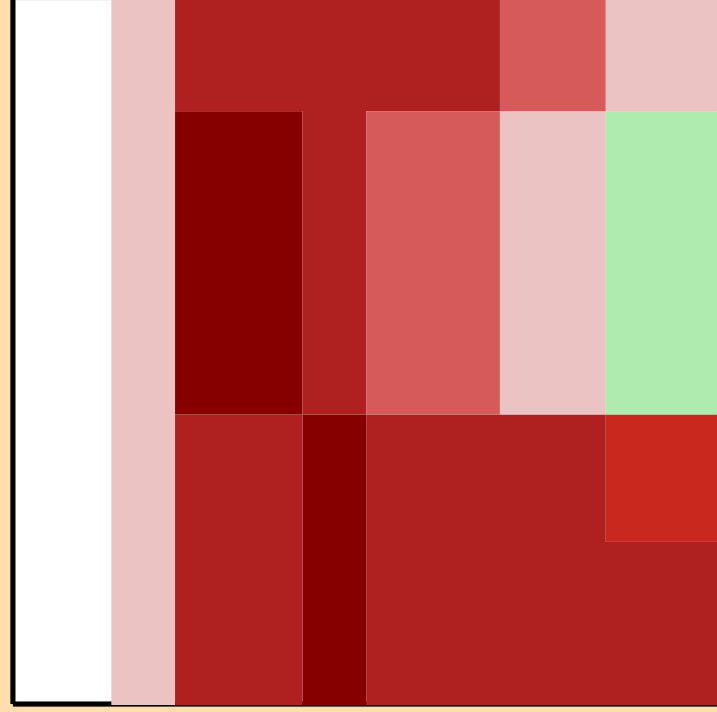
\Delta\sigma/\sigma vs. E for ^{244}\text{Cm}(n,2n)
