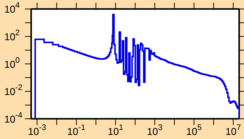
\sigma vs. E for ^{244}\text{Cm}(n,\gamma)
