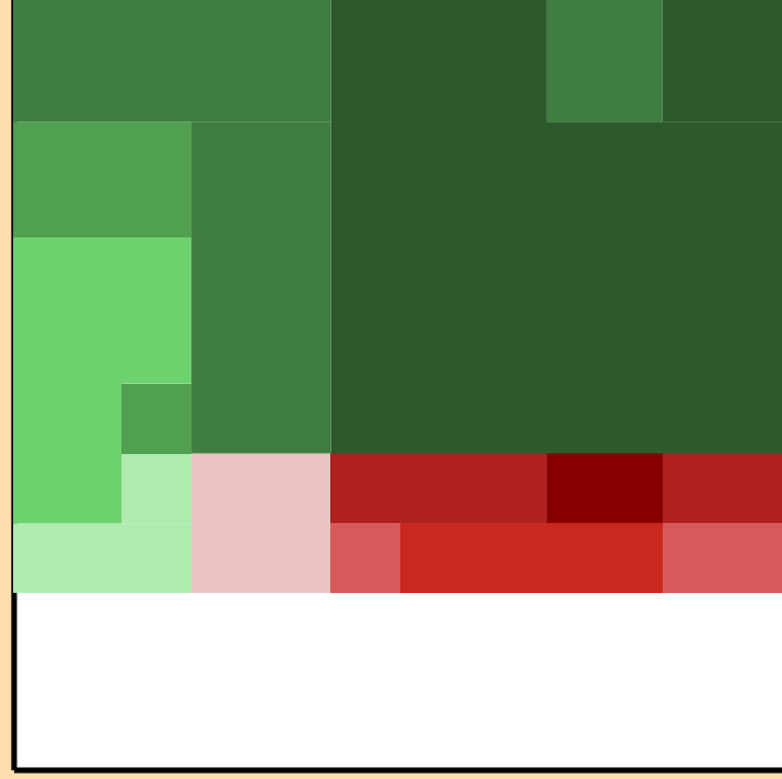
\Delta\sigma/\sigma vs. E for ^{244}\text{Cm}(n,\text{tot.})
