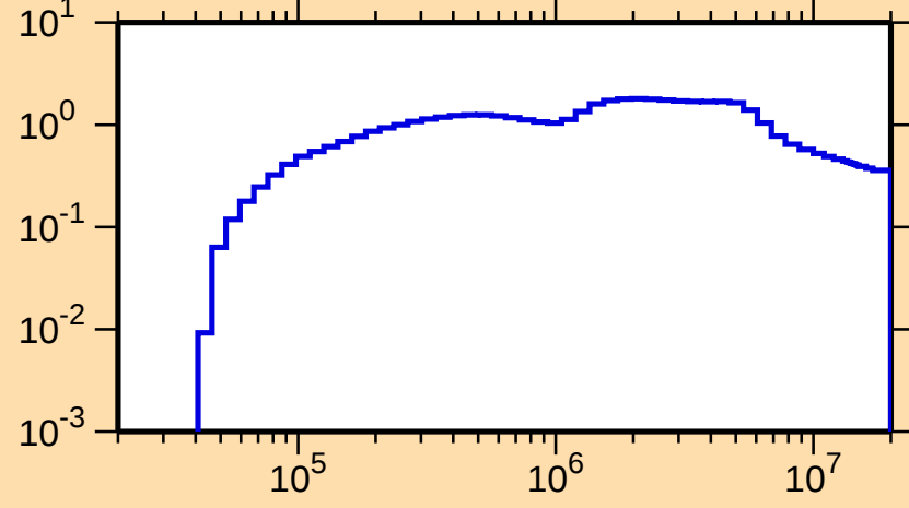
\sigma vs. E for ^{244}\text{Cm}(n,\text{inel.})
