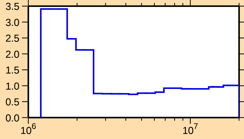
\Delta\sigma/\sigma vs. E for ^{244}\text{Cm}(n,n\text{onel.})
