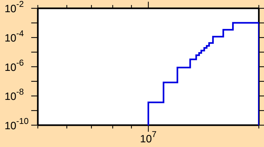
\sigma vs. E for ^{244}\text{Cm}(n,np)
