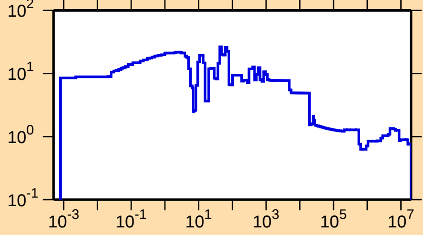
\Delta\sigma/\sigma vs. E for ^{244}\text{Cm}(n,\text{tot.})
