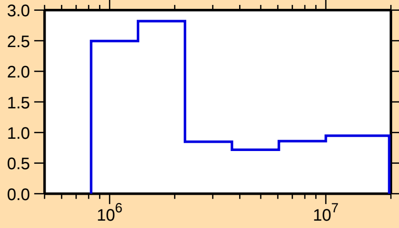
\Delta\sigma/\sigma vs. E for ^{244}\text{Cm}(n,n\text{inel.})
