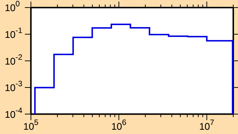
\sigma vs. E for ^{244}\text{Cm}(n,n_2)
