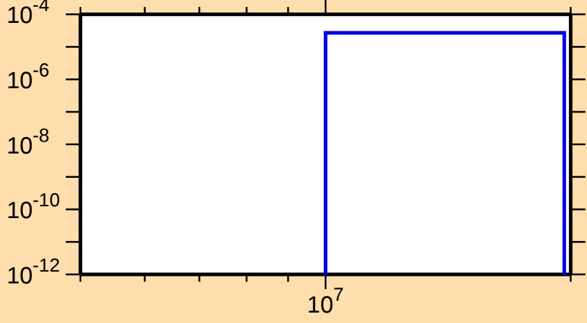
\sigma vs. E for ^{244}\text{Cm}(n,t)
