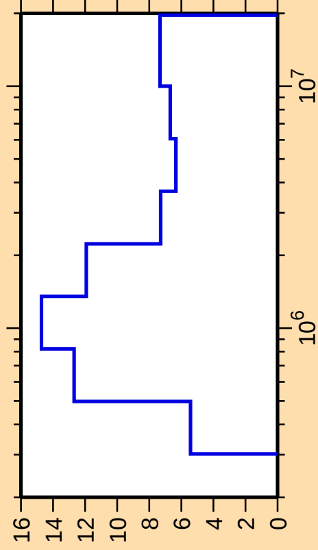
\Delta\sigma/\sigma vs. E for ^{244}\text{Cm}(n,n_3)
