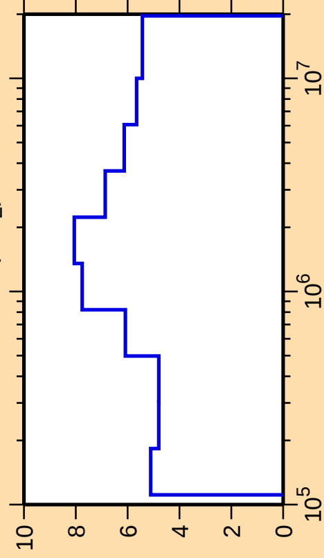
\Delta\sigma/\sigma vs. E for ^{244}\text{Cm}(n,n_2)
