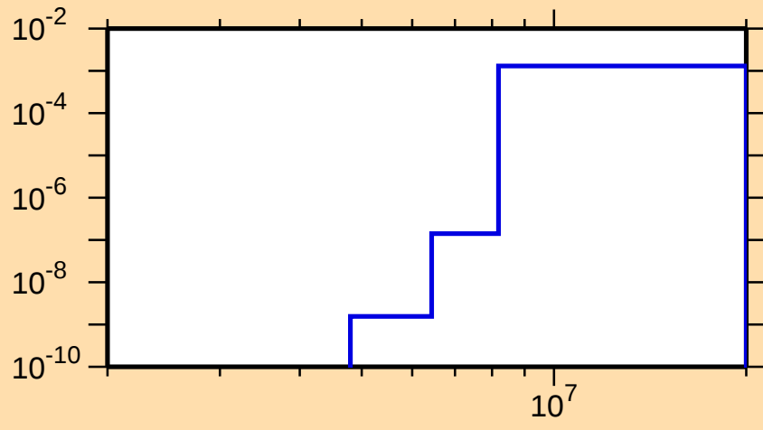
\sigma vs. E for ^{244}\text{Cm}(n,p)
