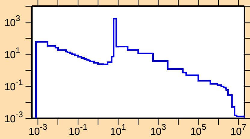
\sigma vs. E for ^{244}\text{Cm}(n,\gamma)
