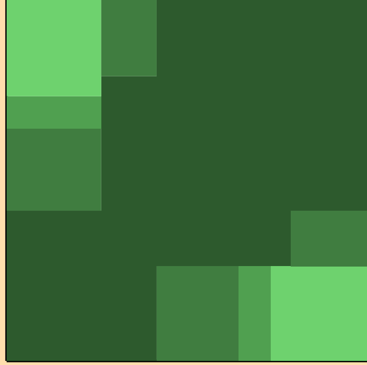
\sigma vs. E for ^{244}\text{Cm}(n,n_2)
