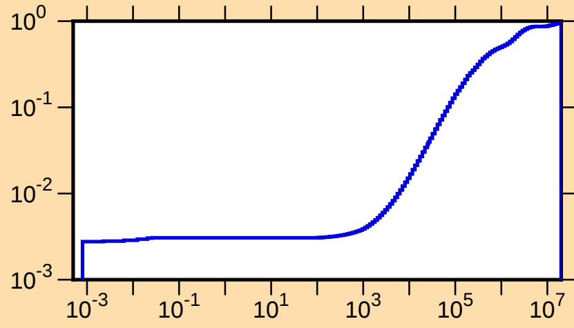
\mu vs. E for ^{245}\text{Cm}(\text{mt251})
