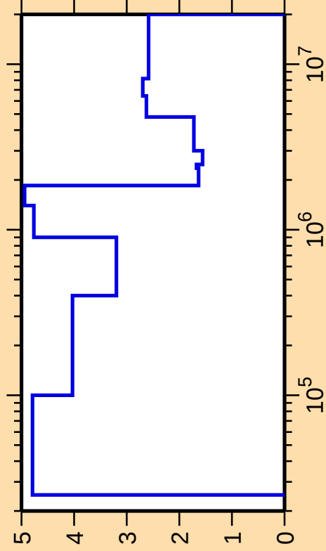
\Delta\sigma/\sigma vs. E for ^{245}\text{Cm}(n,n_1)
