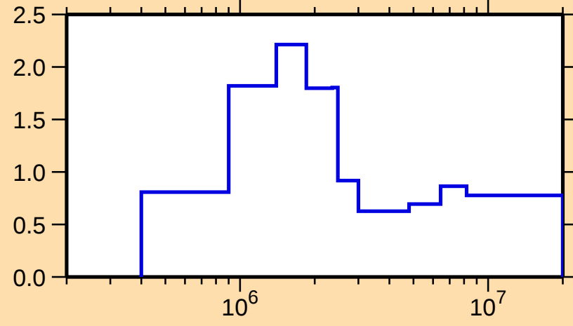
\Delta\sigma/\sigma vs. E for ^{245}\text{Cm}(n,n\text{onel.})
