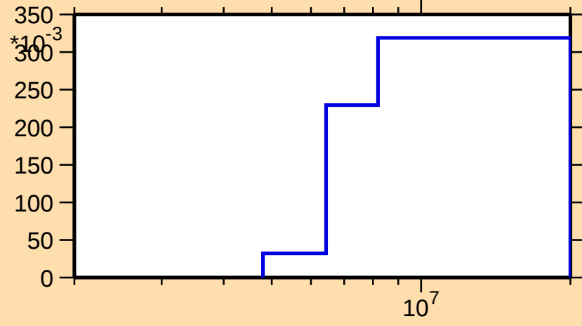
\sigma vs. E for ^{245}\text{Cm}(n,2n)
