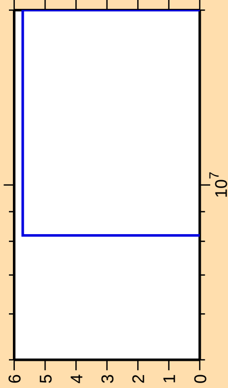
\Delta\sigma/\sigma vs. E for ^{245}\text{Cm}(n,np)
