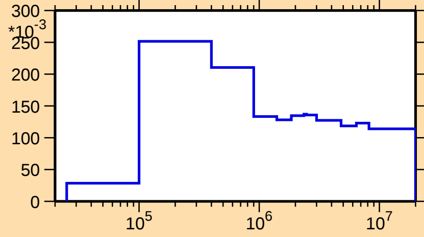
\sigma vs. E for ^{245}\text{Cm}(n,n_1)
