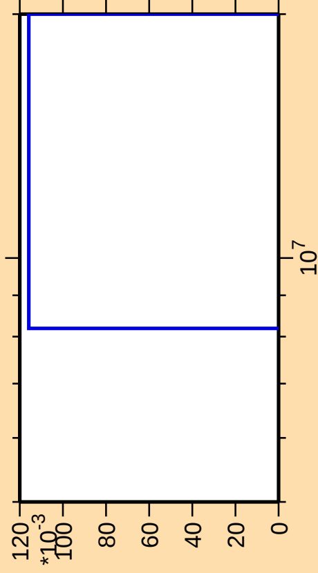
\Delta\sigma/\sigma vs. E for ^{245}\text{Cm}(n,3n\alpha)
