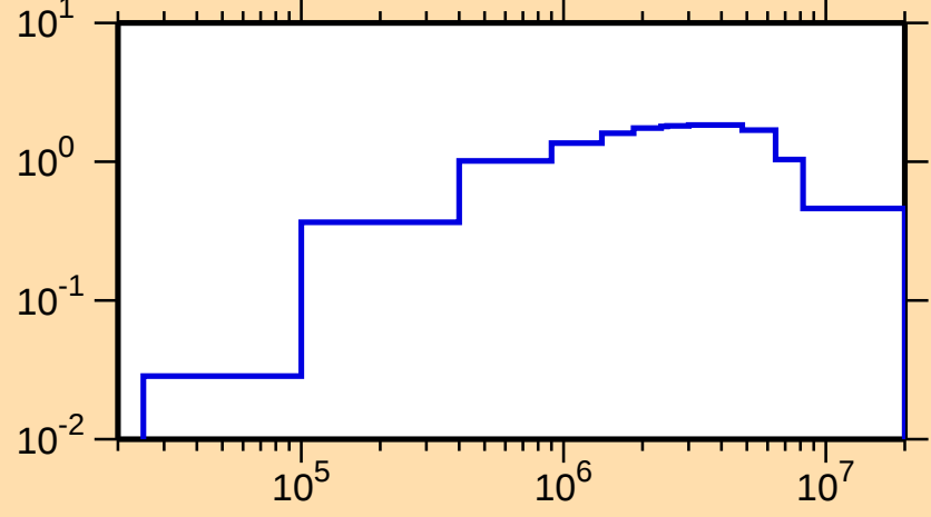
\sigma vs. E for ^{245}\text{Cm}(n,\text{inel.})
