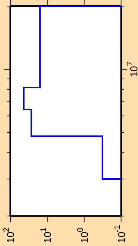
\Delta\sigma/\sigma vs. E for ^{245}\text{Cm}(n,n\alpha)
