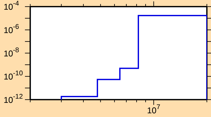
\sigma vs. E for ^{245}\text{Cm}(n,n\alpha)
