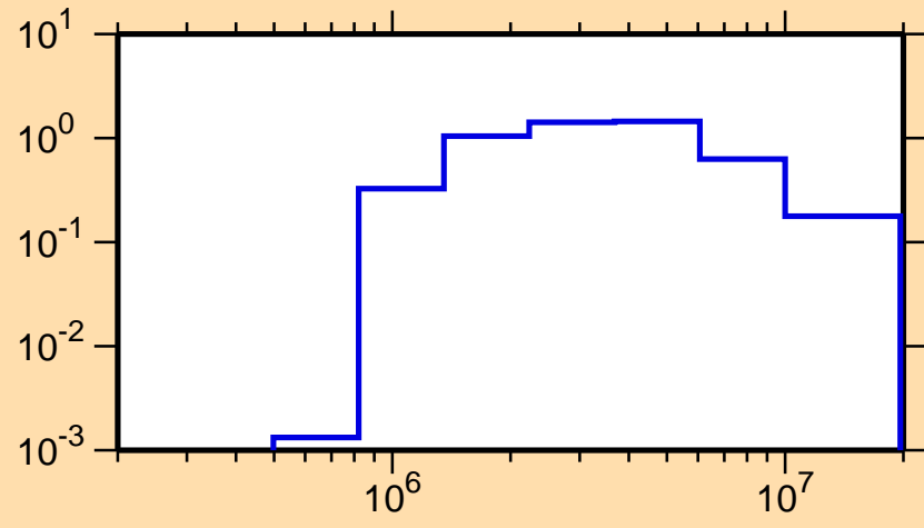
\sigma vs. E for ^{247}\text{Cm}(n,n\text{cont.})
