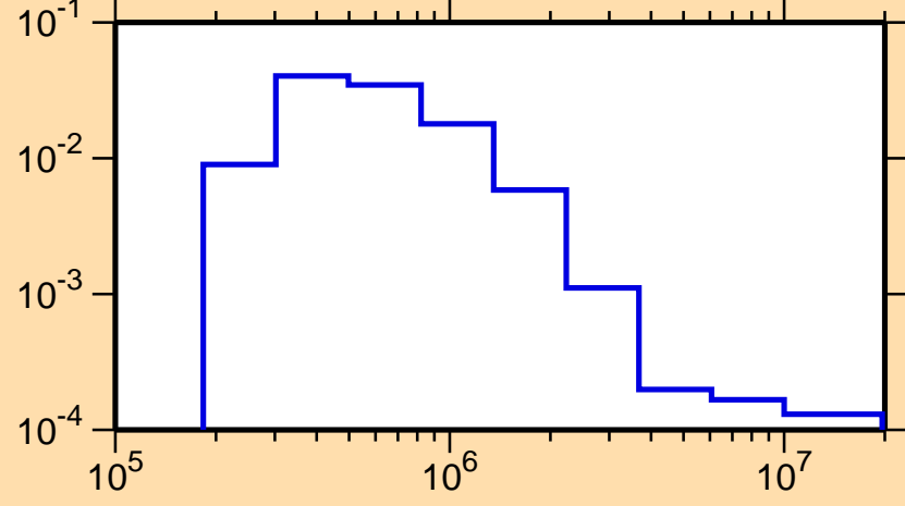
\sigma vs. E for ^{247}\text{Cm}(n,n_4)
