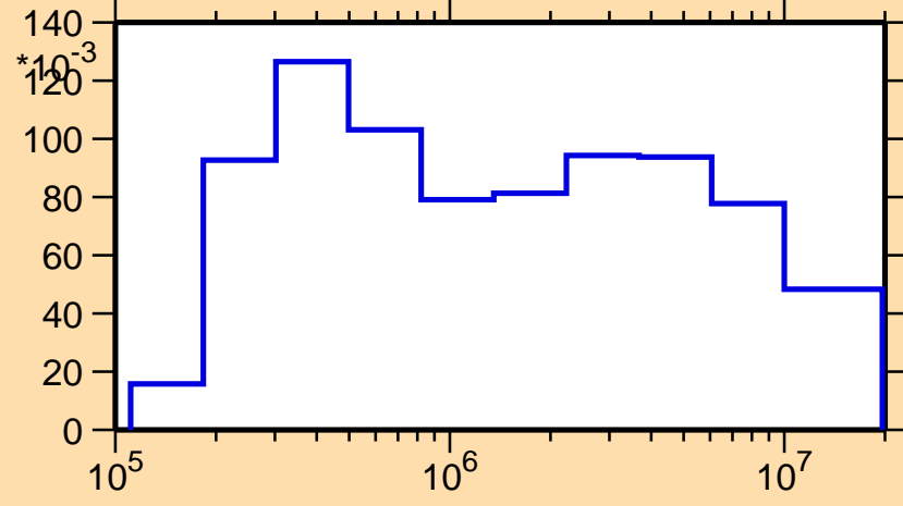
\sigma vs. E for ^{247}\text{Cm}(n,n_2)
