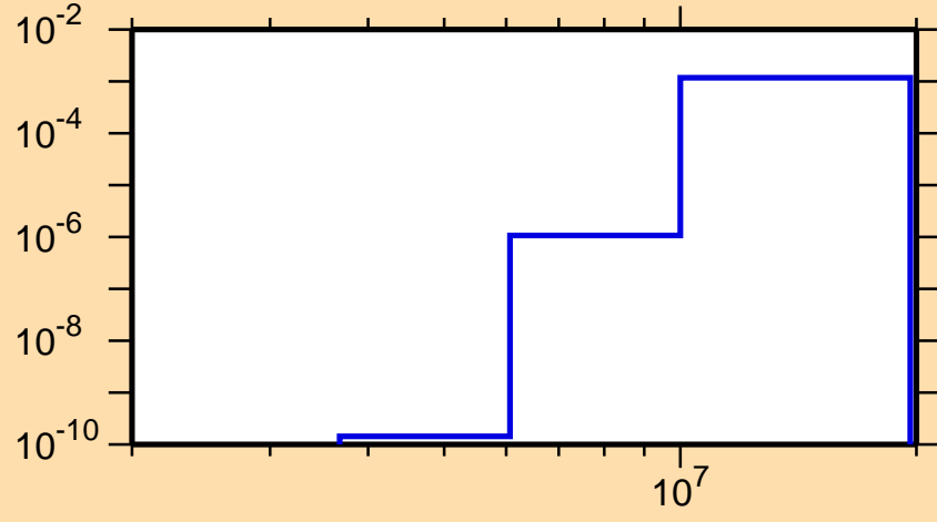
\sigma vs. E for ^{247}\text{Cm}(n,p)
