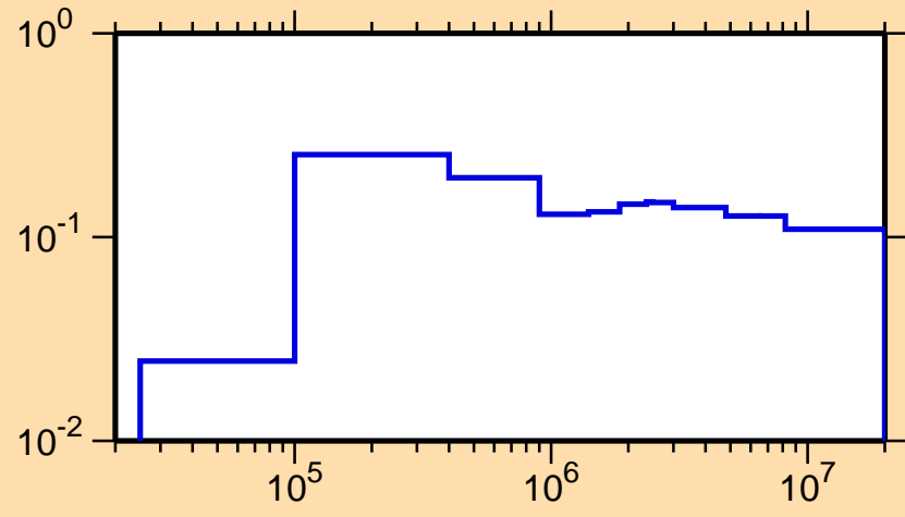
\sigma vs. E for ^{247}\text{Cm}(n,n_1)
