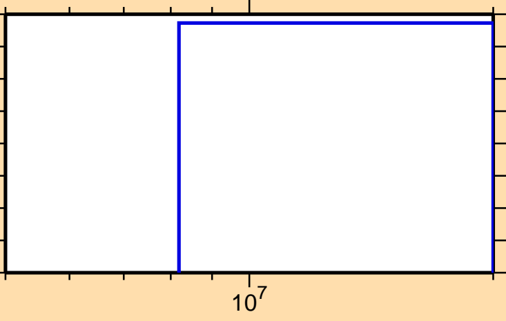
\sigma vs. E for ^{247}\text{Cm}(n,3n)
