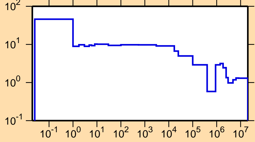
\Delta\sigma/\sigma vs. E for ^{247}\text{Cm}(n,\text{nonel.})
