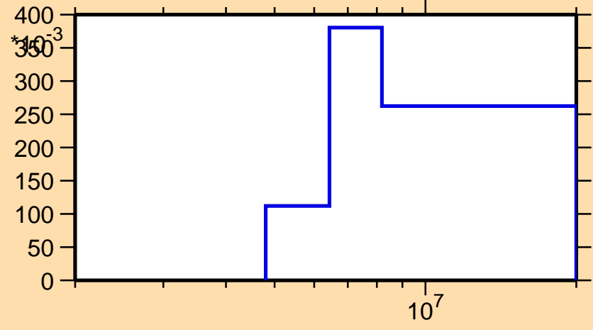
\sigma vs. E for ^{247}\text{Cm}(n,2n)
