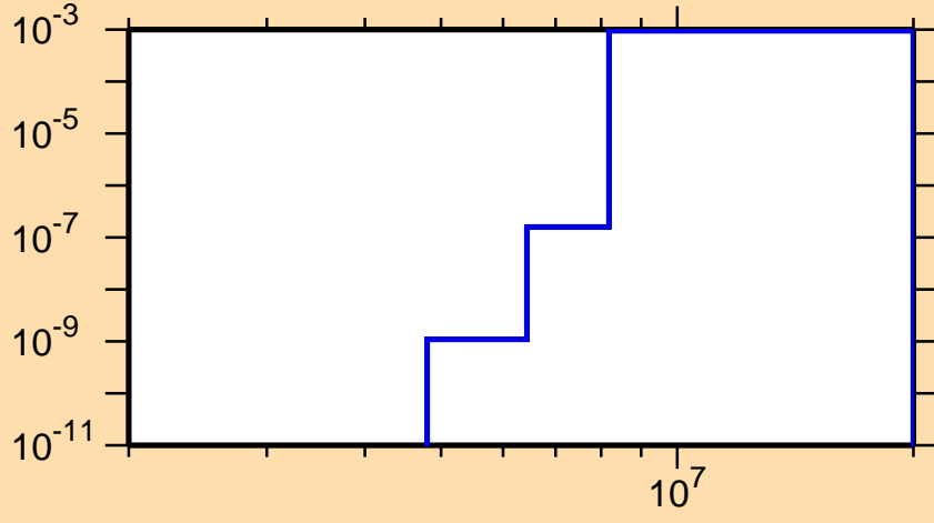
\sigma vs. E for ^{247}\text{Cm}(n,p)
