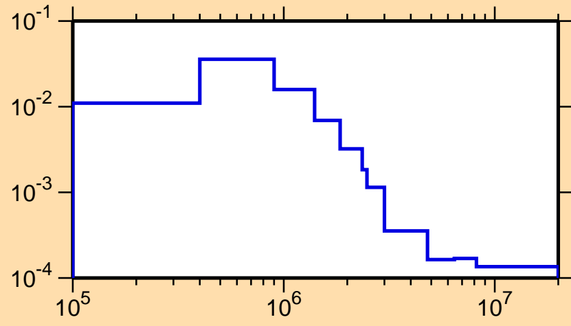
\sigma vs. E for ^{247}\text{Cm}(n,n_4)
