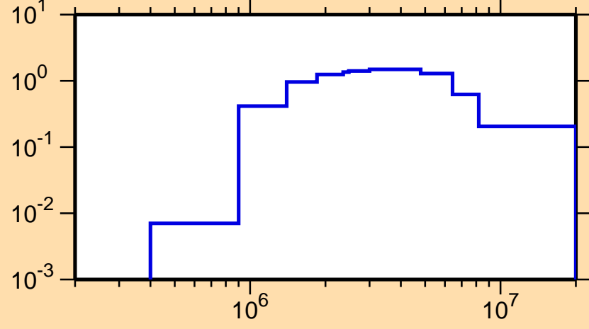
\sigma vs. E for ^{247}\text{Cm}(n,n\text{cont.})
