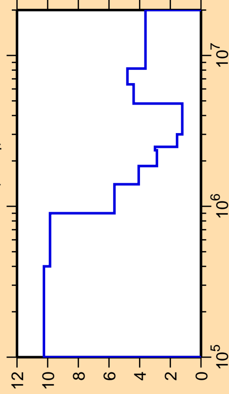
\Delta\sigma/\sigma vs. E for ^{247}\text{Cm}(n,n_4)
