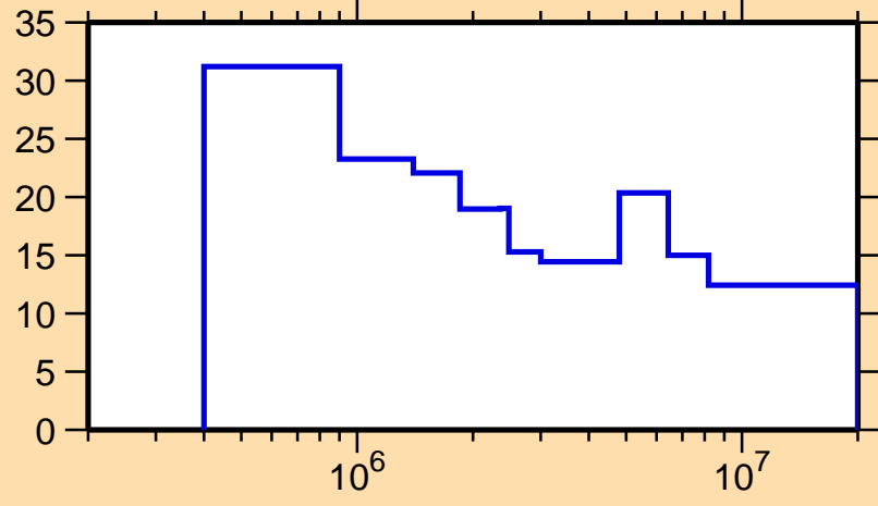
\Delta\sigma/\sigma vs. E for ^{247}\text{Cm}(n,n\text{cont.})
