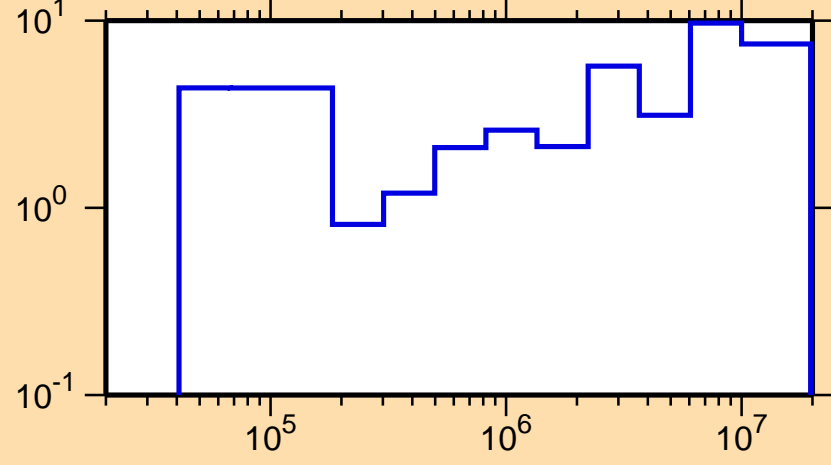
\Delta\sigma/\sigma vs. E for ^{248}\text{Cm}(n,\text{inel.})
