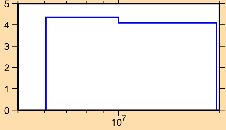
\Delta\sigma/\sigma vs. E for ^{248}\text{Cm}(n,p)
