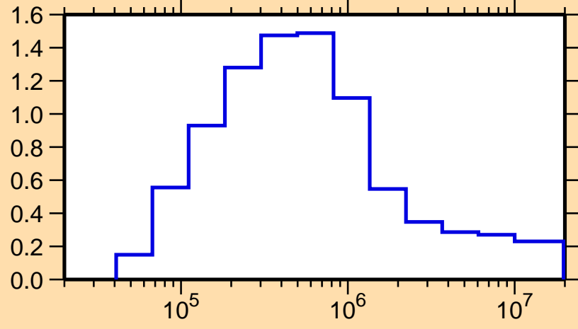
\sigma vs. E for ^{248}\text{Cm}(n,n_1)
