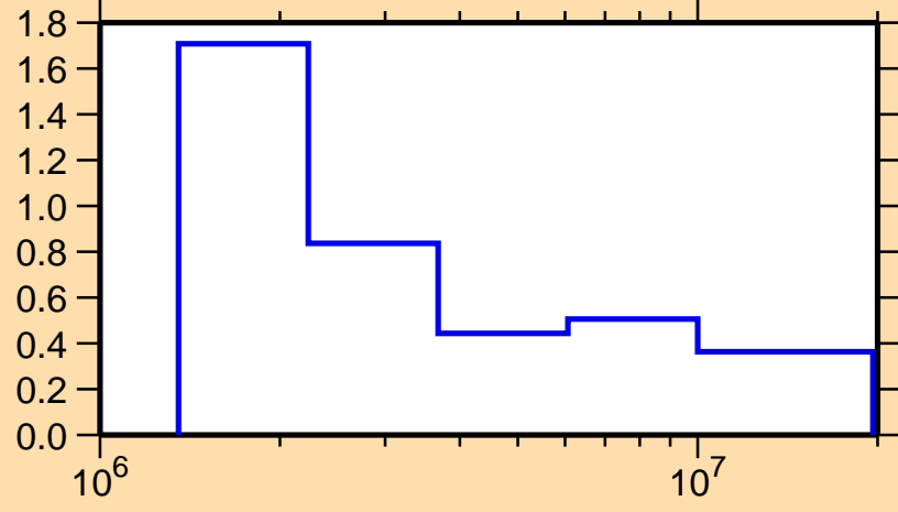
\Delta\sigma/\sigma vs. E for ^{248}\text{Cm}(n,n\text{onel.})
