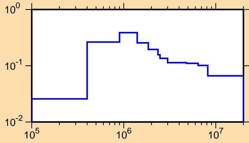
\sigma vs. E for ^{248}\text{Cm}(n,n_2)
