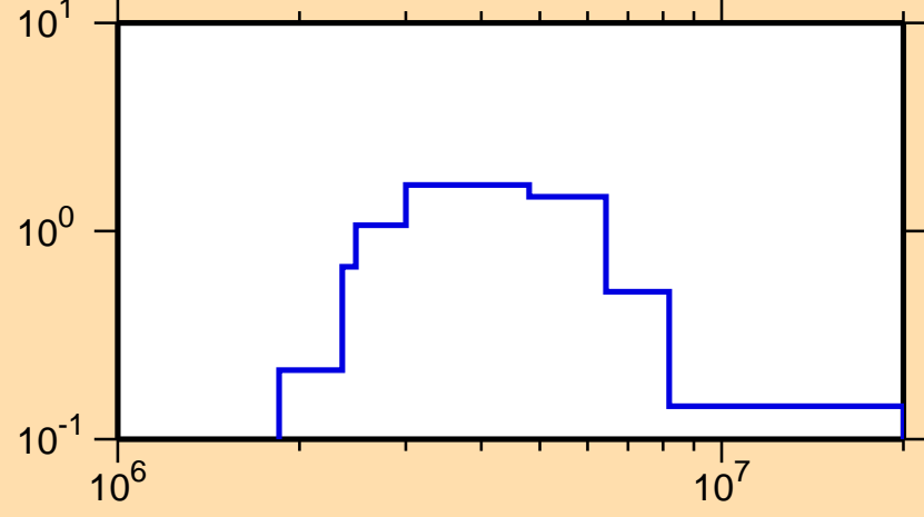
\sigma vs. E for ^{248}\text{Cm}(n,n\text{cont.})
