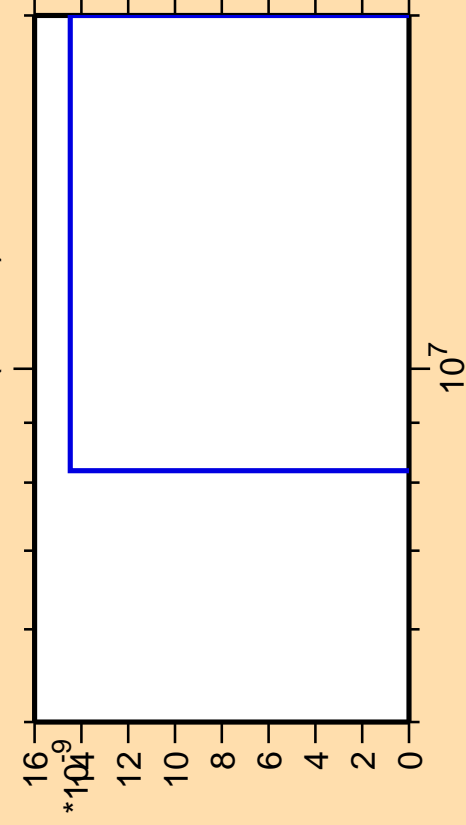
\Delta\sigma/\sigma vs. E for ^{248}\text{Cm} (mt 42)
