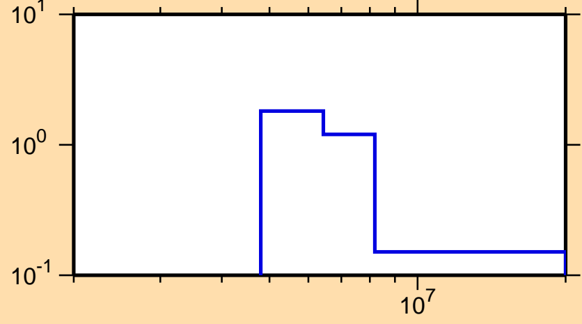
\Delta\sigma/\sigma vs. E for ^{248}\text{Cm}(n,el.)
