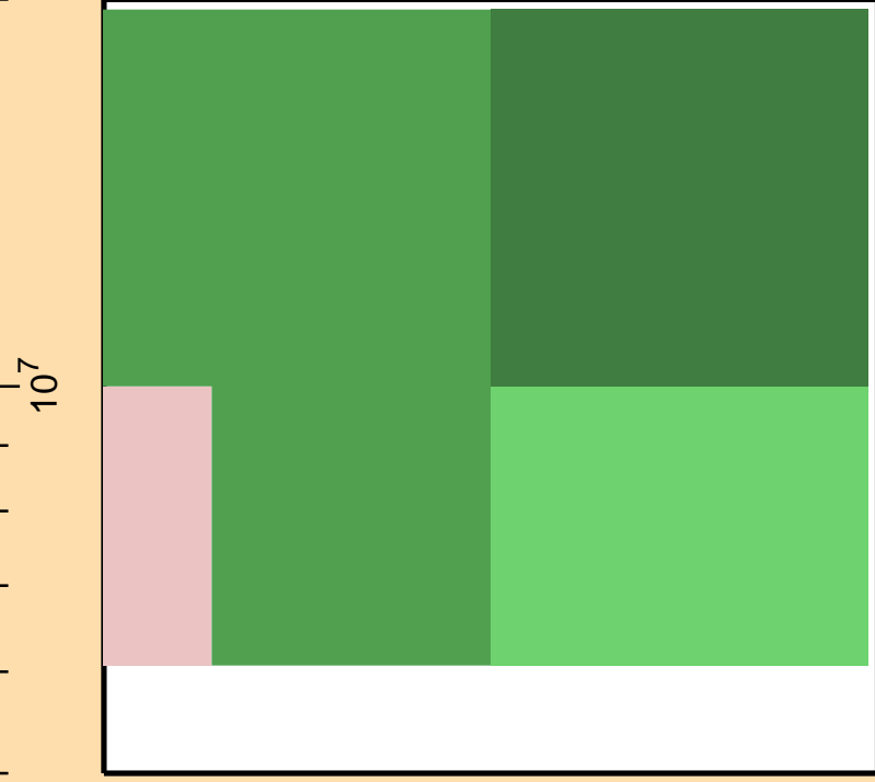
\Delta\sigma/\sigma vs. E for ^{250}\text{Cm}(n,\gamma)
