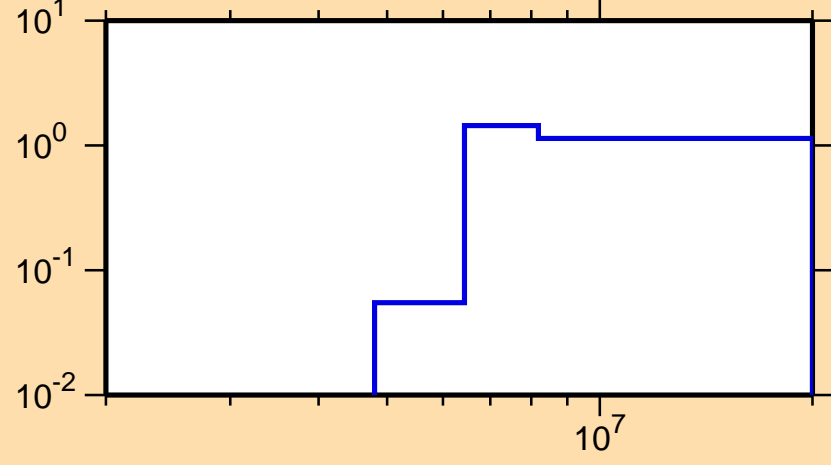
\sigma vs. E for ^{250}\text{Cm}(n,2n)
