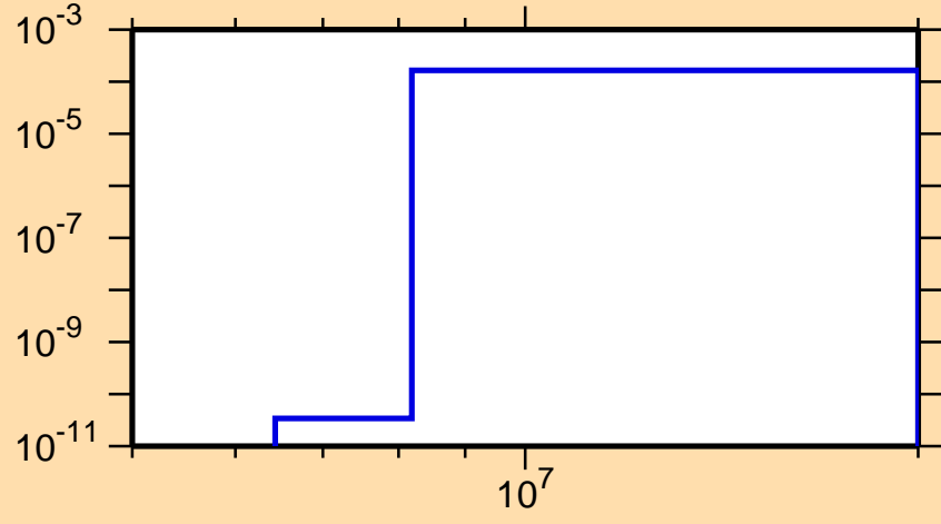
\sigma vs. E for ^{250}\text{Cm}(n,p)
