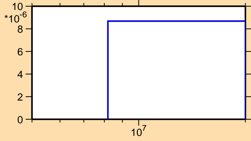
\sigma vs. E for ^{250}\text{Cm}(n,d)
