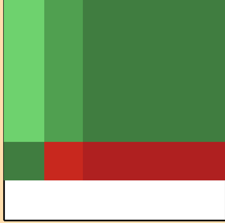
\Delta\sigma/\sigma vs. E for ^{250}\text{Cm}(n,\gamma)
