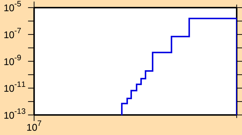
\sigma vs. E for ^{251}\text{Cm}(n,\text{nd})
