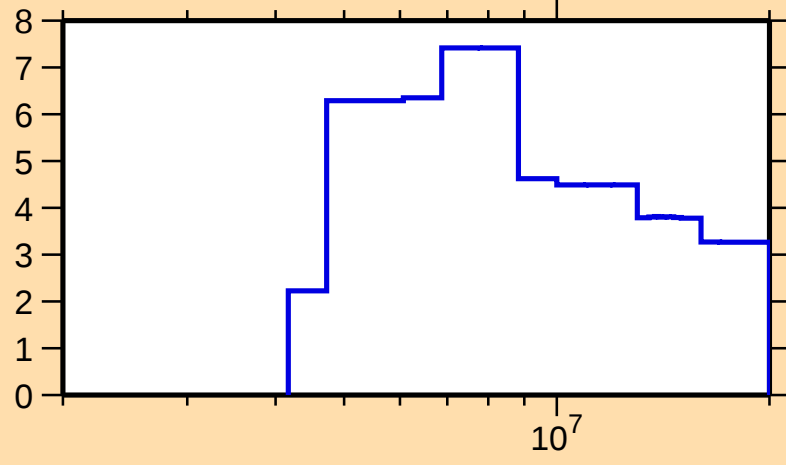
\Delta\sigma/\sigma vs. E for ^{251}\text{Cm}(n,\text{tot.})
