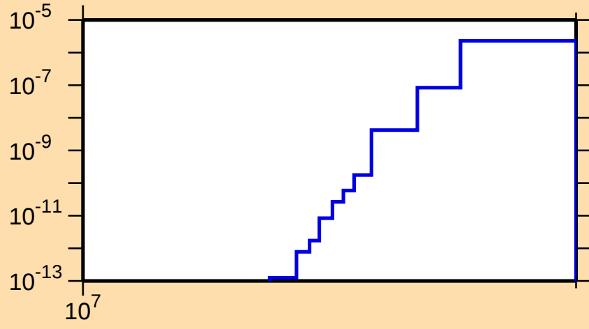
\sigma vs. E for ^{251}\text{Cm}(n,nt)
