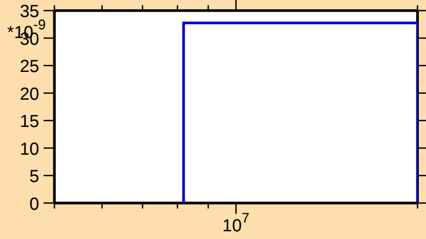
\sigma vs. E for ^{251}\text{Cm}(n,2n\alpha)
