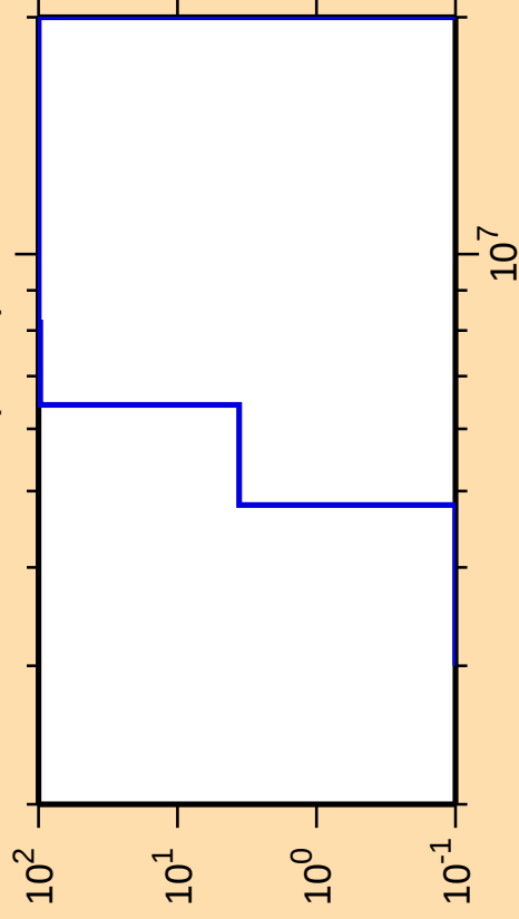
\Delta\sigma/\sigma vs. E for ^{251}\text{Cm}(n,n\alpha)
