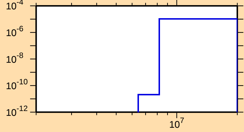
\sigma vs. E for ^{251}\text{Cm}(n,n\alpha)
