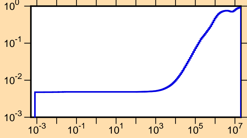
\mu vs. E for ^{142}\text{Dy}(\text{mt251})
