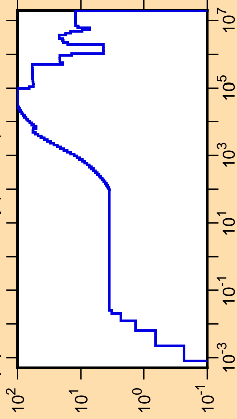
\Delta\mu/\mu vs. E for ^{142}\text{Dy}(\text{mt251})
