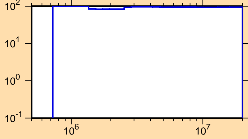
\Delta\sigma/\sigma vs. E for ^{142}\text{Dy}(n,ncont.)
