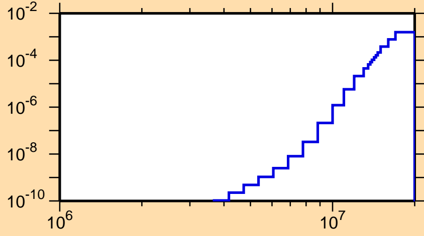
\sigma vs. E for ^{142}\text{Dy}(n,\text{He3})
