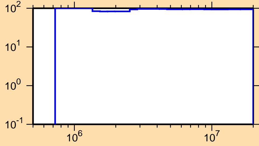
\Delta\sigma/\sigma vs. E for ^{142}\text{Dy}(n,ncont.)
