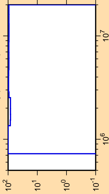
\Delta\sigma/\sigma vs. E for ^{142}\text{Dy}(n,\text{ncont.})
