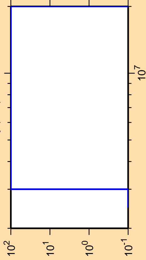
\Delta\sigma/\sigma vs. E for ^{142}\text{Dy}(n,d)
