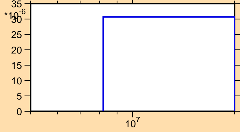
\sigma vs. E for ^{142}\text{Dy}(n,t)
