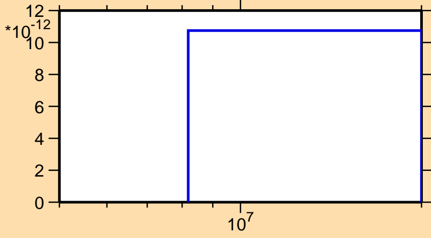
\sigma vs. E for ^{142}\text{Dy}(\text{mt } 34)
