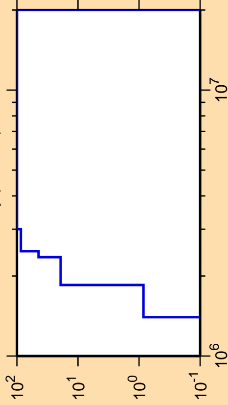
\Delta\sigma/\sigma vs. E for ^{142}\text{Dy}(n,\text{He3})
