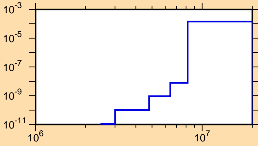
\sigma vs. E for ^{142}\text{Dy}(n,\text{He3})
