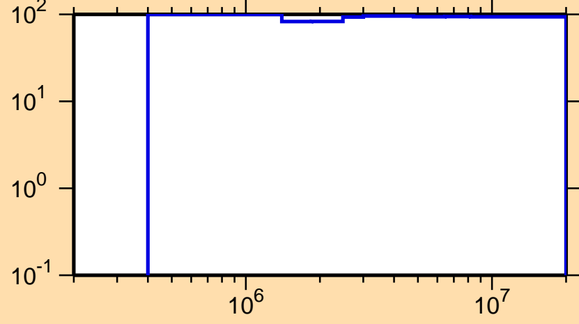
\Delta\sigma/\sigma vs. E for ^{142}\text{Dy}(n,n\text{cont.})
