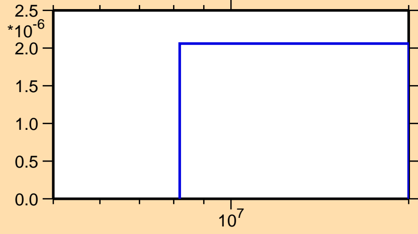
\sigma vs. E for ^{142}\text{Dy} (mt 45)
