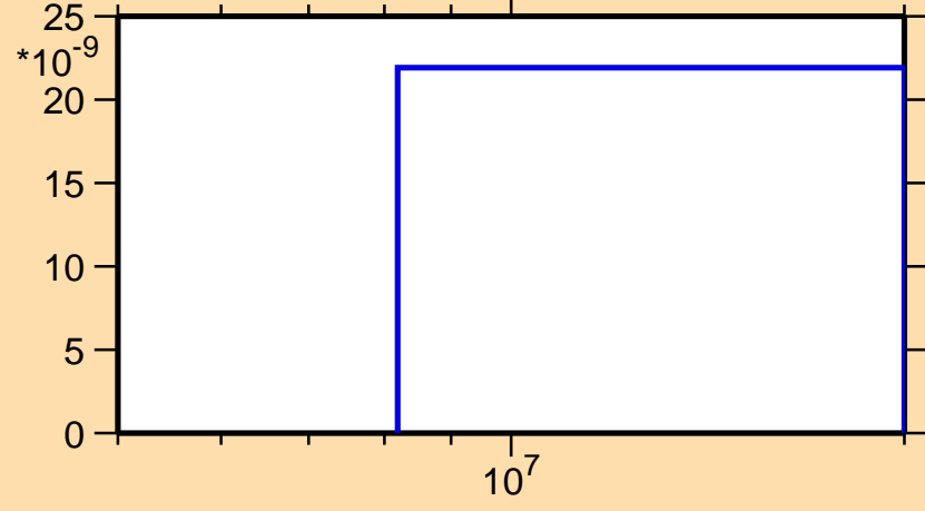
\sigma vs. E for ^{142}\text{Dy}(n,2np)
