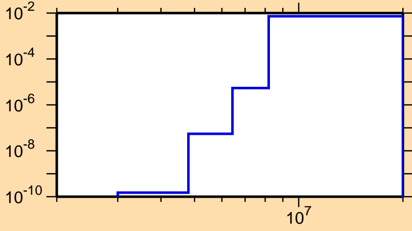
\sigma vs. E for ^{142}\text{Dy}(n,d)
