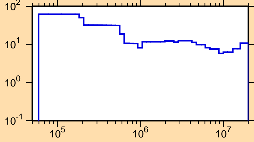
\Delta\sigma/\sigma vs. E for ^{143}\text{Dy}(n,\text{el.})
