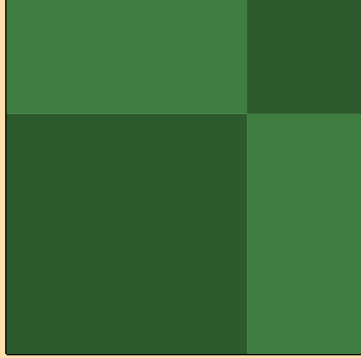
\sigma vs. E for ^{143}\text{Dy}(n,2n)
