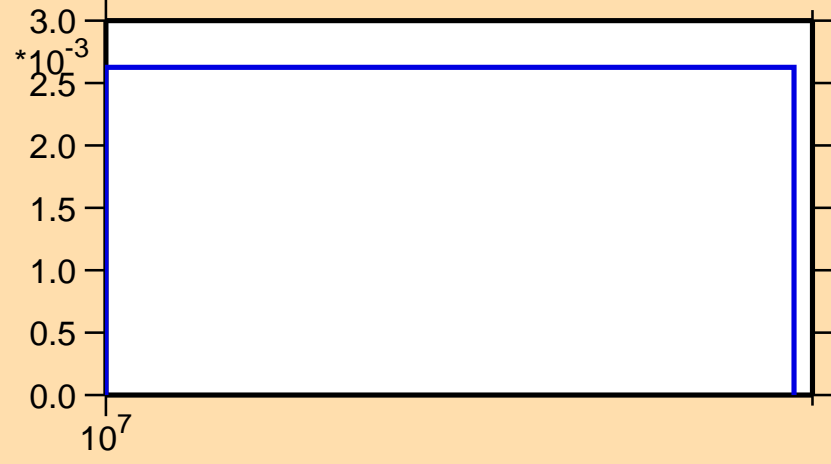
\sigma vs. E for ^{143}\text{Dy}(n,2n)
