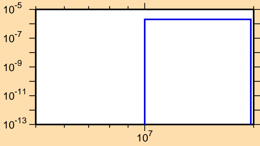
\sigma vs. E for ^{143}\text{Dy} (mt 45)
