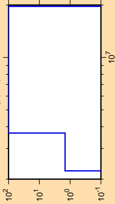
\Delta\sigma/\sigma vs. E for ^{143}\text{Dy}(n,d)
