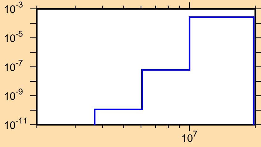
\sigma vs. E for ^{143}\text{Dy}(n,\text{He3})
