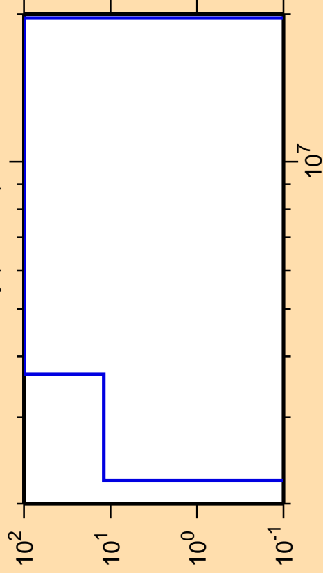
\Delta\sigma/\sigma vs. E for ^{143}\text{Dy}(n,\text{He3})
