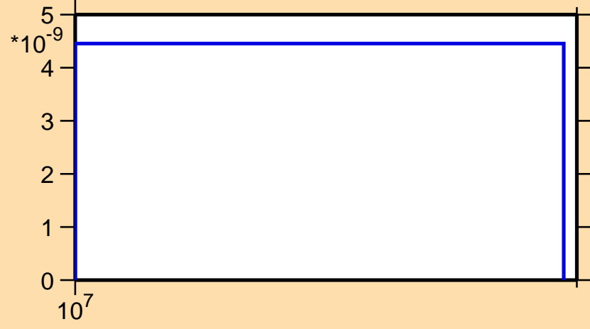
\sigma vs. E for ^{143}\text{Dy}(n,\text{nd})
