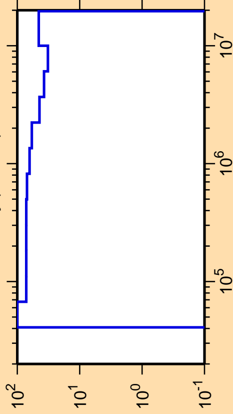
\Delta\sigma/\sigma vs. E for ^{143}\text{Dy}(n,\text{inel.})
