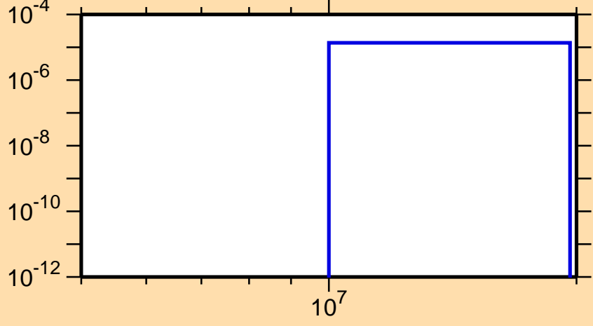
\sigma vs. E for ^{143}\text{Dy}(n,\text{pt})
