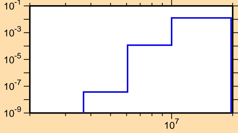
\sigma vs. E for ^{143}\text{Dy}(n,d)
