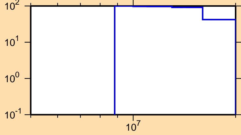
\Delta\sigma/\sigma vs. E for ^{143}\text{Dy}(n,2n)
