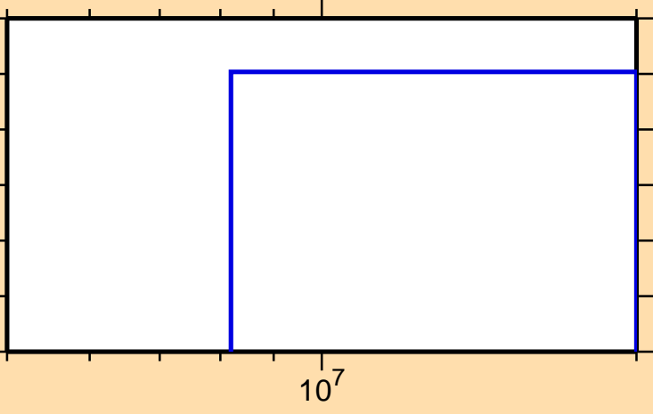
\sigma vs. E for ^{143}\text{Dy}(\text{mt117})
