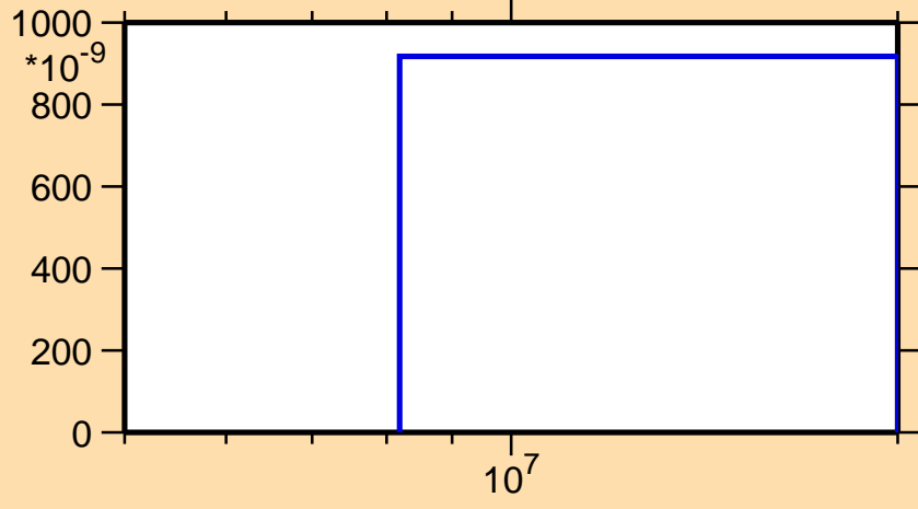
\sigma vs. E for ^{143}\text{Dy} (mt 45)
