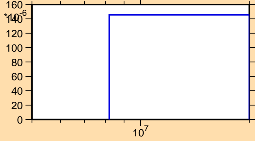
\sigma vs. E for ^{143}\text{Dy}(n,t)
