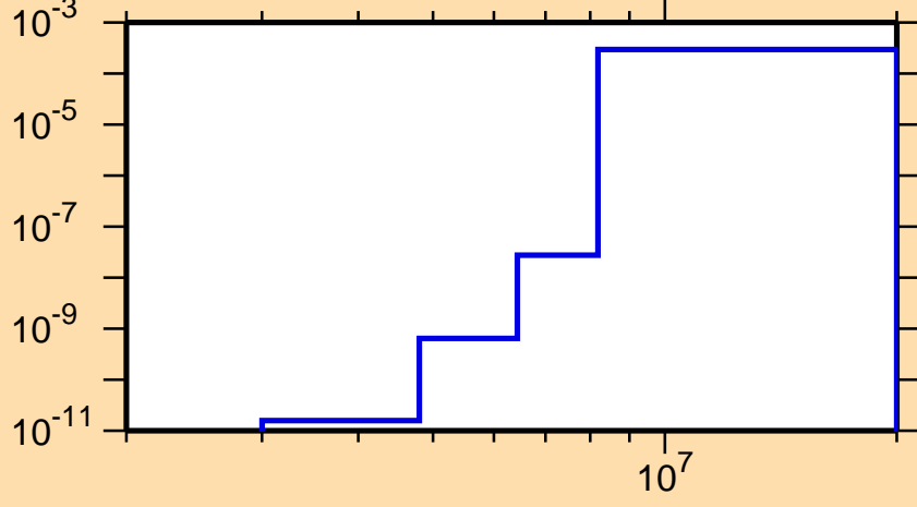
\sigma vs. E for ^{143}\text{Dy}(n,\text{He3})
