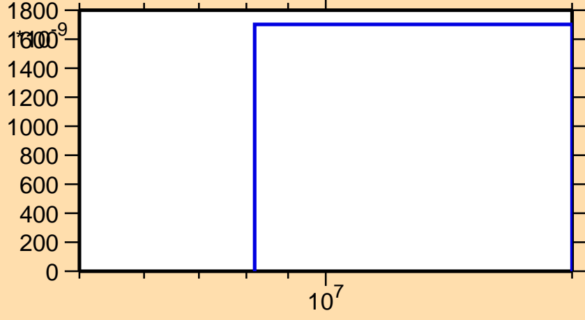
\sigma vs. E for ^{143}\text{Dy}(n,2np)
