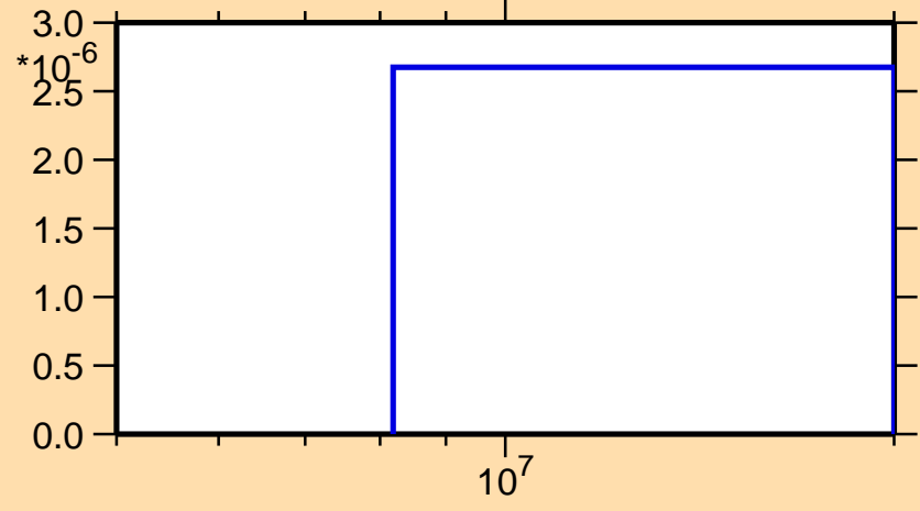
\sigma vs. E for ^{143}\text{Dy}(n,2n\alpha)
