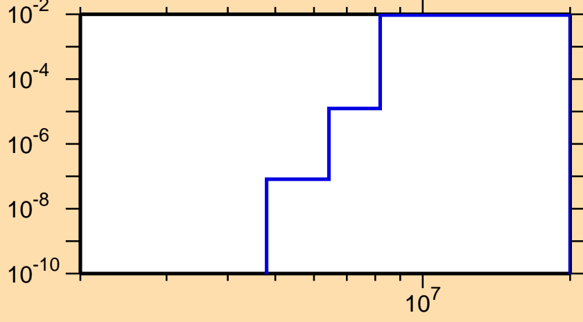
\sigma vs. E for ^{145}\text{Dy}(n,d)
