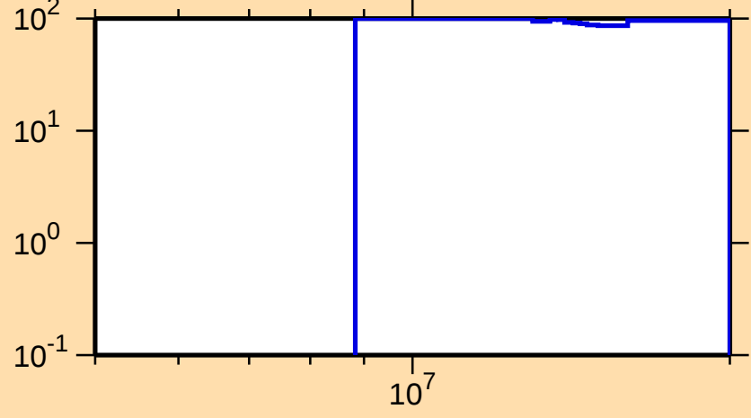
\Delta\sigma/\sigma vs. E for ^{145}\text{Dy}(n,2n)
