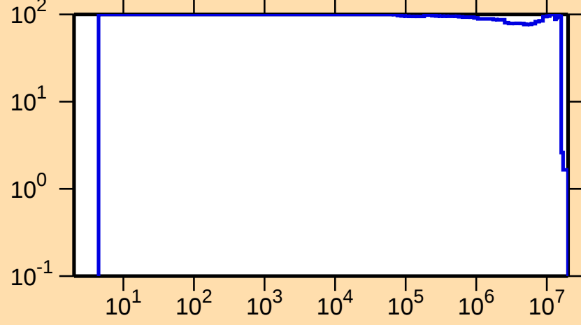
\Delta\sigma/\sigma vs. E for ^{145}\text{Dy}(n,n_1)
