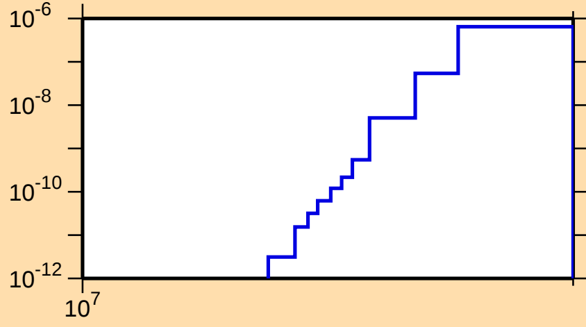
\sigma vs. E for ^{145}\text{Dy}(n,2n\alpha)
