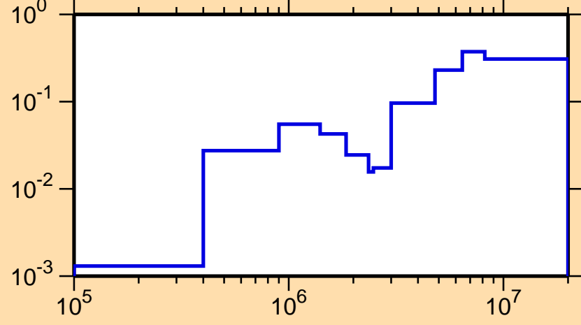
\sigma vs. E for ^{145}\text{Dy}(n,\text{inel.})
