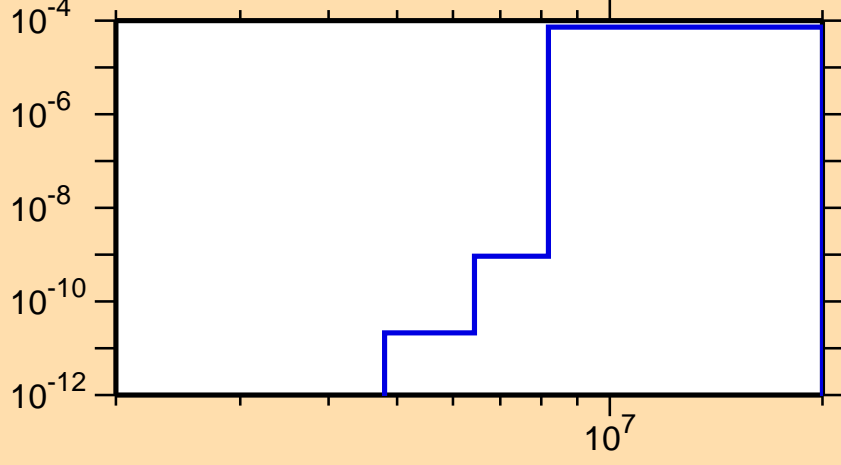
\sigma vs. E for ^{145}\text{Dy}(n,\text{He3})
