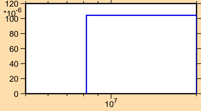
\sigma vs. E for ^{145}\text{Dy}(n,t)
