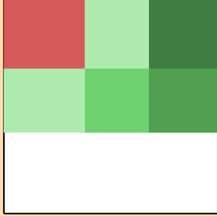
\Delta\sigma/\sigma vs. E for ^{146}\text{Dy}(n,\text{el.})
