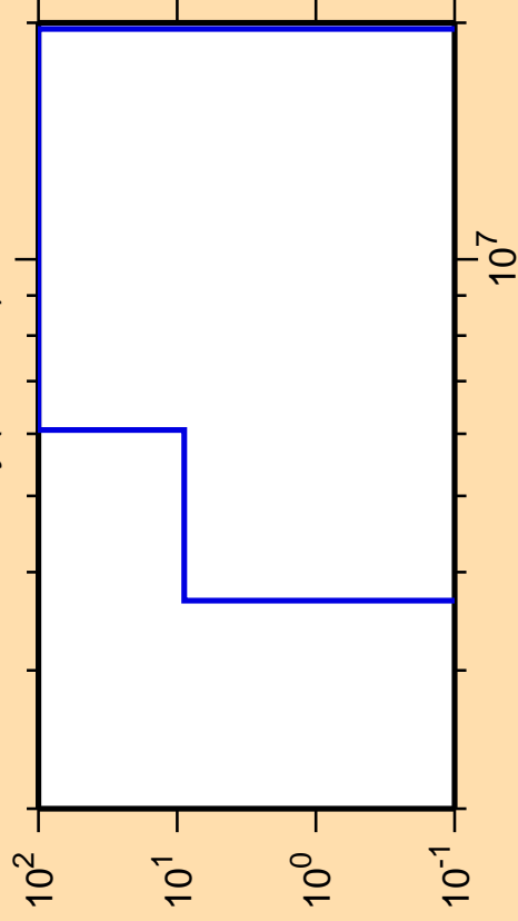
\Delta\sigma/\sigma vs. E for ^{146}\text{Dy}(n,\text{He3})
