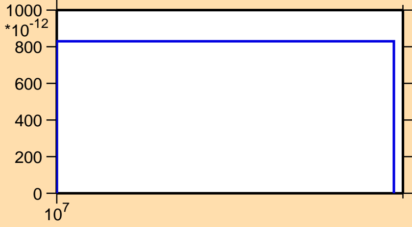
\sigma vs. E for ^{146}\text{Dy}(n,\text{pt})
