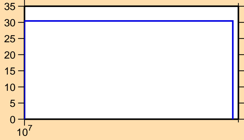
\Delta\sigma/\sigma vs. E for ^{146}\text{Dy}(n,\text{el.})
