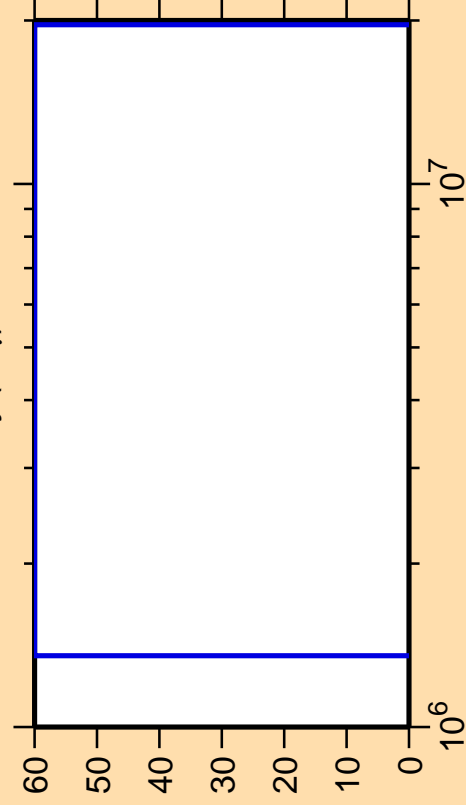
\Delta\sigma/\sigma vs. E for ^{146}\text{Dy}(n,\gamma)
