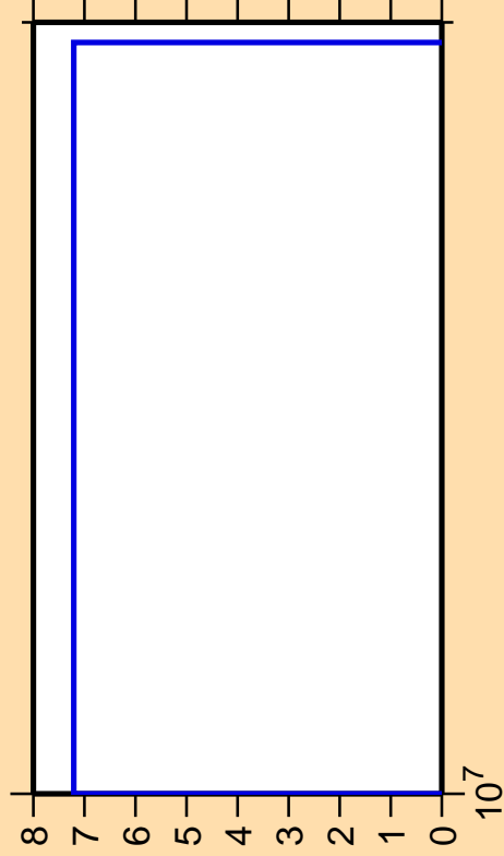
\Delta\sigma/\sigma vs. E for ^{146}\text{Dy} (mt 34)
