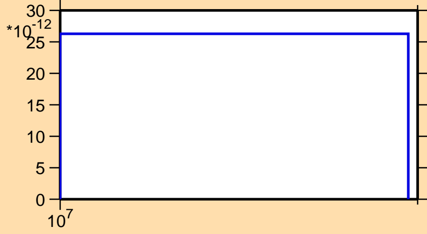
\sigma vs. E for ^{146}\text{Dy}(n,2n\alpha)
