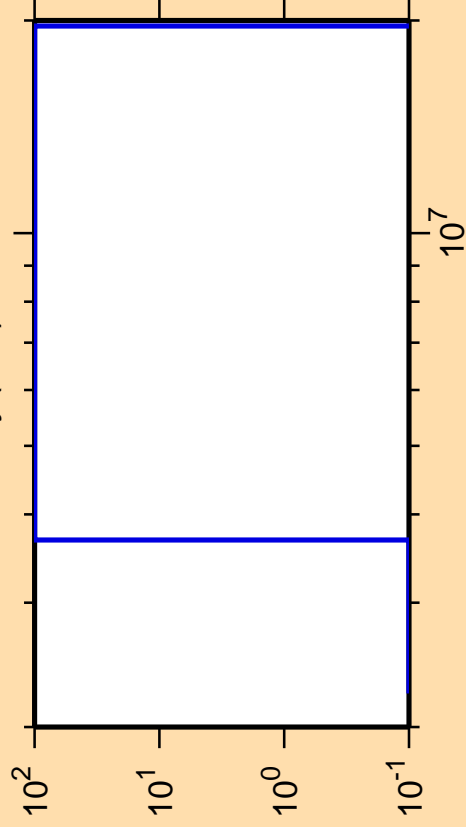
\Delta\sigma/\sigma vs. E for ^{146}\text{Dy}(n,d)
