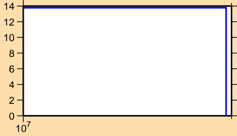
\Delta\sigma/\sigma vs. E for ^{146}\text{Dy}(n,\text{tot.})
