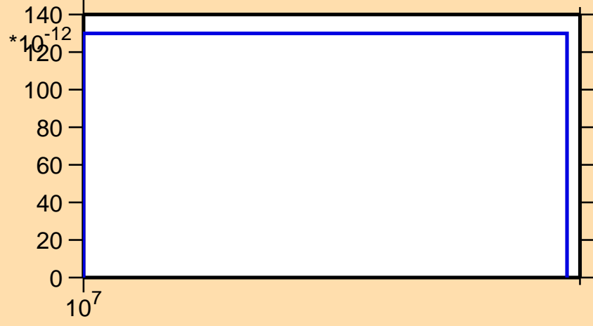
\sigma vs. E for ^{146}\text{Dy}(n,\text{nd})
