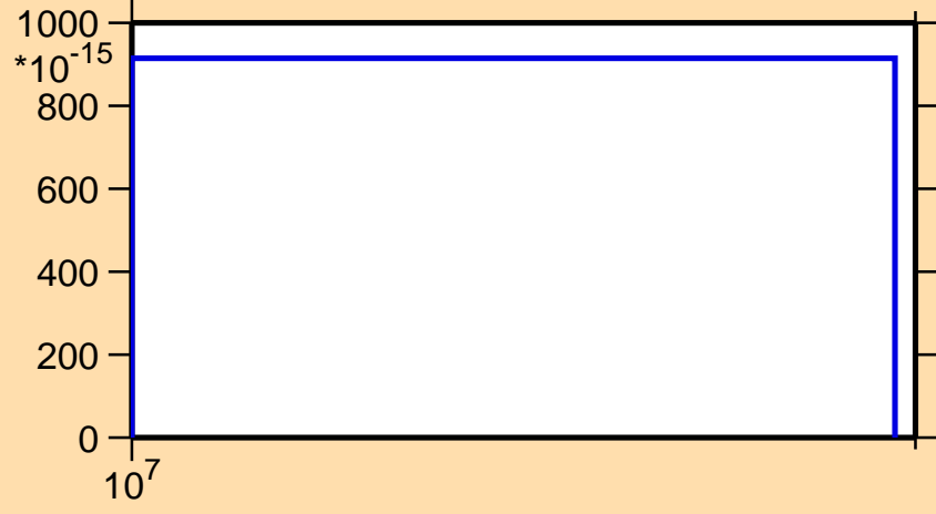
\sigma vs. E for ^{146}\text{Dy} (mt 34)
