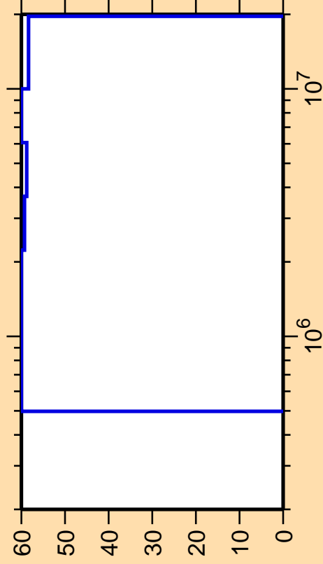
\Delta\sigma/\sigma vs. E for ^{146}\text{Dy}(n,\text{inel.})
