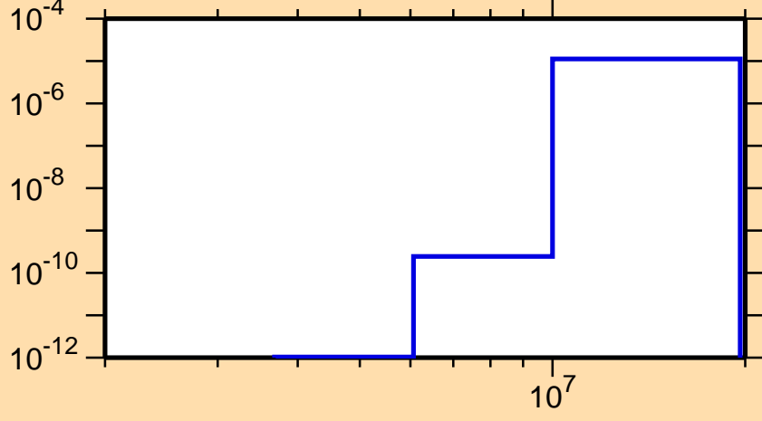
\sigma vs. E for ^{146}\text{Dy}(n,\text{He3})
