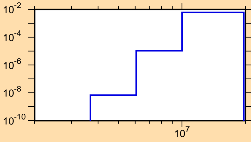
\sigma vs. E for ^{146}\text{Dy}(n,d)
