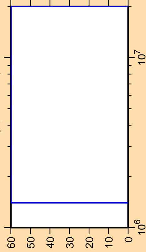
\Delta\sigma/\sigma vs. E for ^{146}\text{Dy}(n,ncont.)
