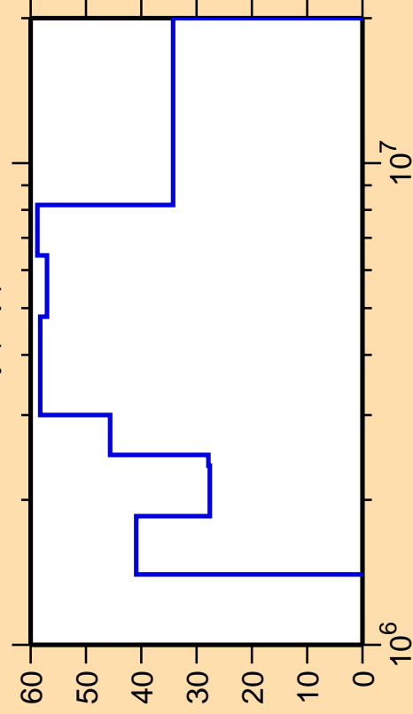
\Delta\sigma/\sigma vs. E for ^{146}\text{Dy}(n,p)
