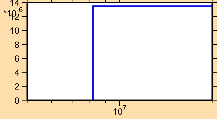
\sigma vs. E for ^{146}\text{Dy}(n,t)
