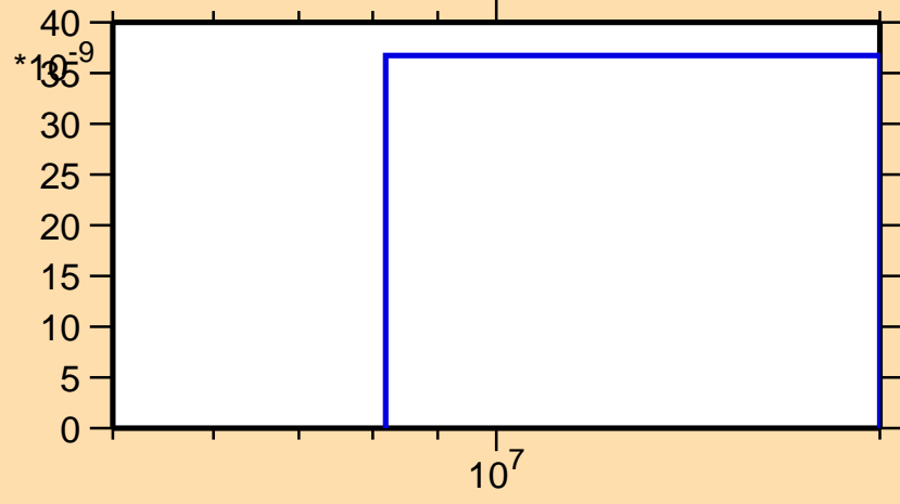
\sigma vs. E for ^{146}\text{Dy}(\text{mt } 45)
