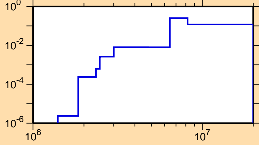
\sigma vs. E for ^{146}\text{Dy}(n,ncont.)
