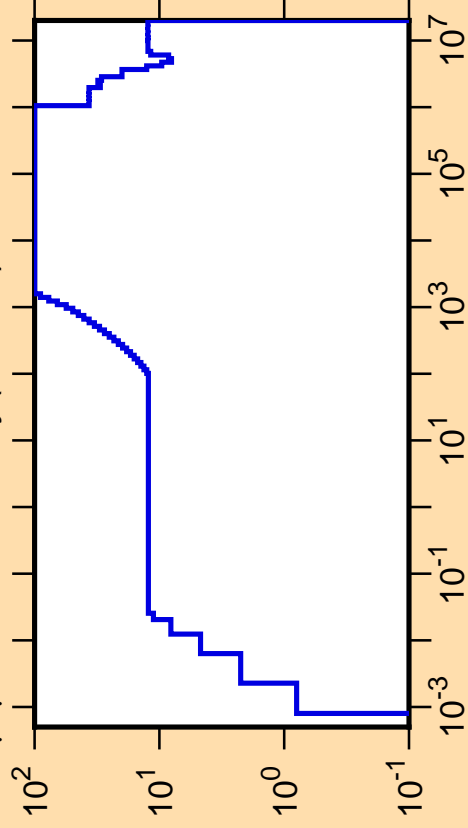
\Delta\mu/\mu vs. E for ^{147}\text{Dy}(\text{mt251})
