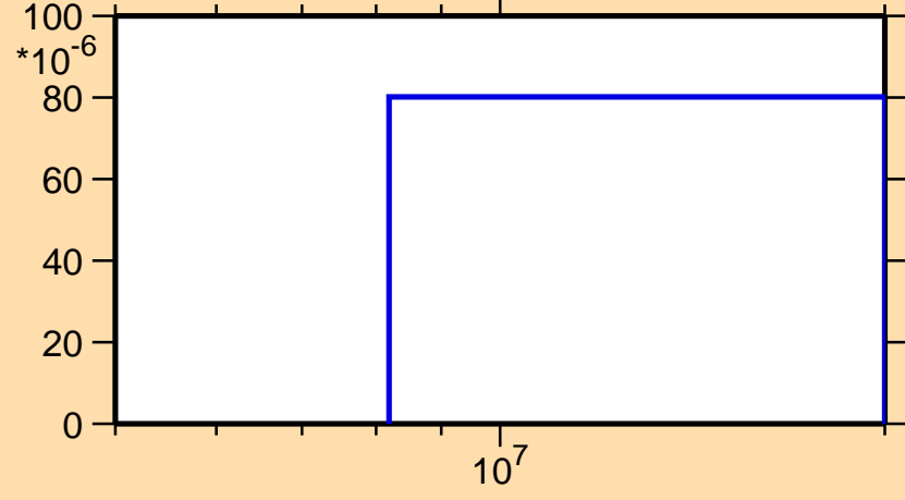
\sigma vs. E for ^{147}\text{Dy}(n,2np)
