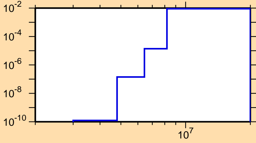
\sigma vs. E for ^{147}\text{Dy}(n,d)
