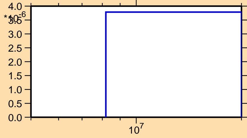
\sigma vs. E for ^{147}\text{Dy}(n,\text{pd})
