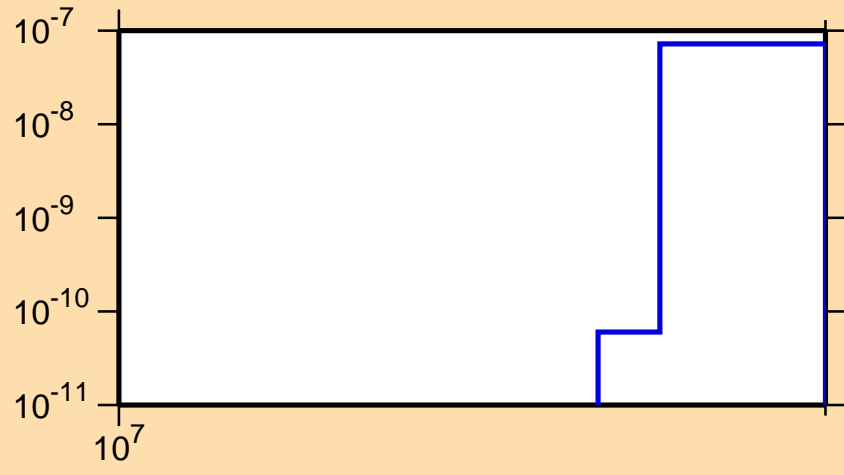
\sigma vs. E for ^{148}\text{Dy}(n,\text{nd})
