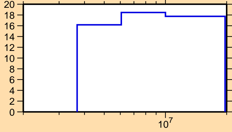
\Delta\sigma/\sigma vs. E for ^{148}\text{Dy}(n,nonel.)
