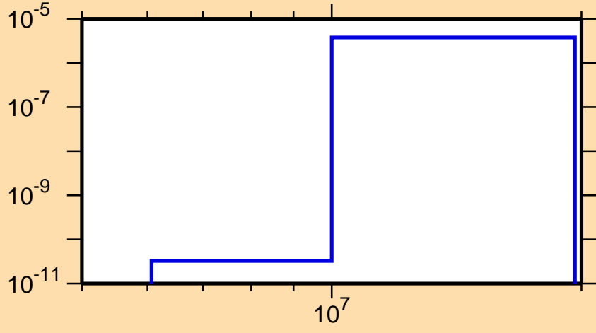
\sigma vs. E for ^{148}\text{Dy}(n,\text{He3})
