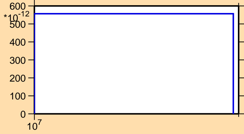
\sigma vs. E for ^{148}\text{Dy}(n,\text{nd})
