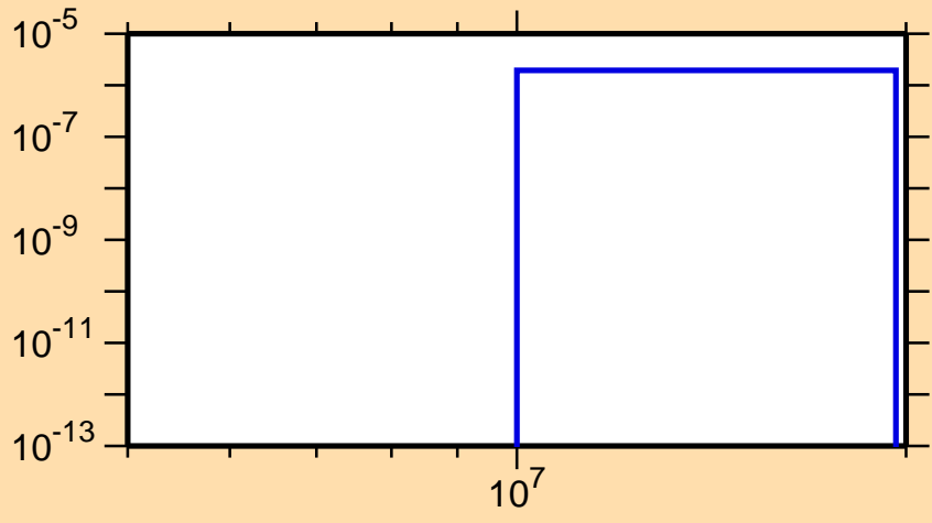
\sigma vs. E for ^{148}\text{Dy}(n,pd)
