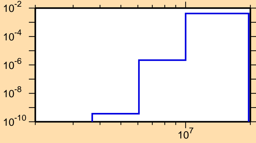
\sigma vs. E for ^{148}\text{Dy}(n,d)
