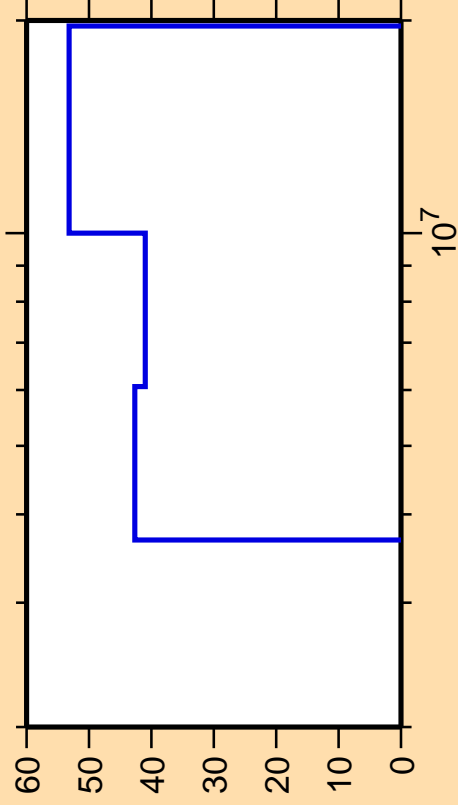
\Delta\sigma/\sigma vs. E for ^{148}\text{Dy}(n,ncont.)
