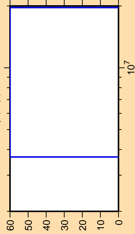
\Delta\sigma/\sigma vs. E for ^{148}\text{Dy}(n,p)
