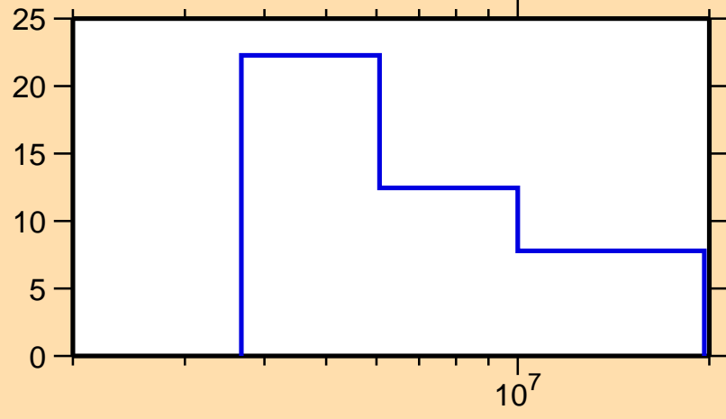
\Delta\sigma/\sigma vs. E for ^{148}\text{Dy}(n,tot.)
