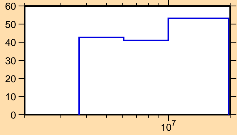
\Delta\sigma/\sigma vs. E for ^{148}\text{Dy}(n,ncont.)
