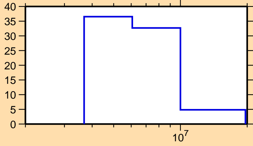
\Delta\sigma/\sigma vs. E for ^{148}\text{Dy}(n,el.)
