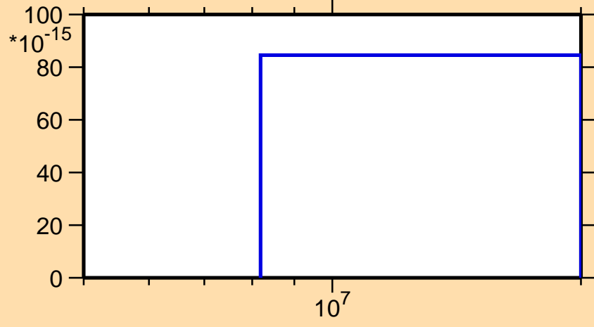
\sigma vs. E for ^{148}\text{Dy}(\text{mt } 34)
