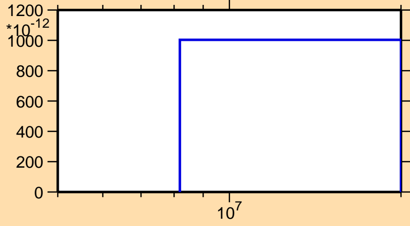
\sigma vs. E for ^{148}\text{Dy}(\text{mt } 45)
