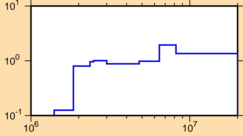
\sigma vs. E for ^{148}\text{Dy}(n,\text{inel.})
