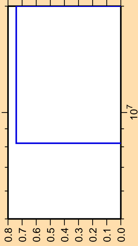
\Delta\sigma/\sigma vs. E for ^{148}\text{Dy}(\text{mt } 34)
