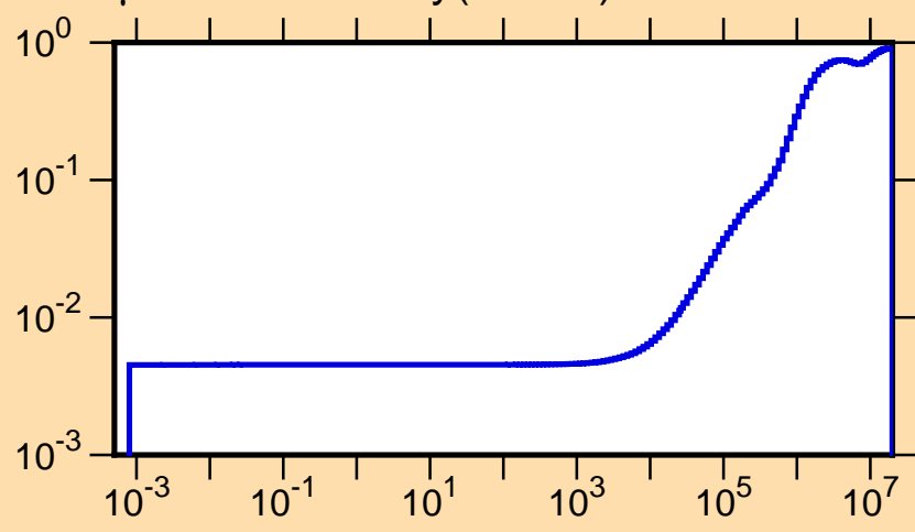
\mu vs. E for ^{149}\text{Dy}(\text{mt251})
