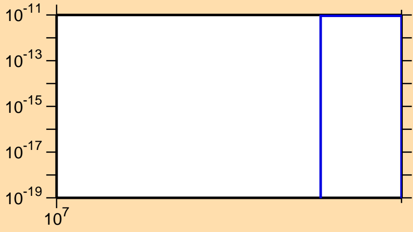
\sigma vs. E for ^{149}\text{Dy}(n,nt)
