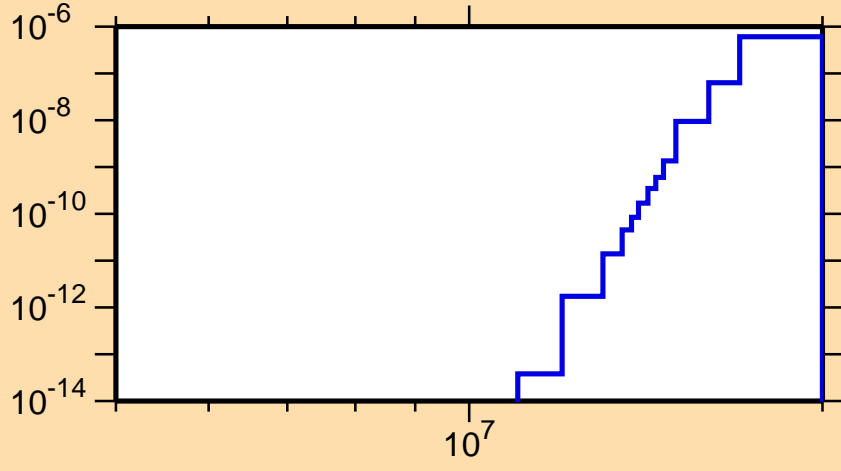
\sigma vs. E for ^{149}\text{Dy}(\text{mt } 45)
