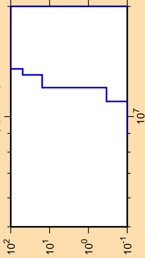
\Delta\sigma/\sigma vs. E for ^{149}\text{Dy}(\text{mt } 45)
