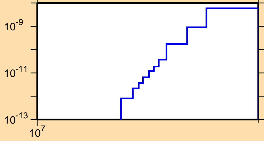
\sigma vs. E for ^{149}\text{Dy}(\text{mt117})
