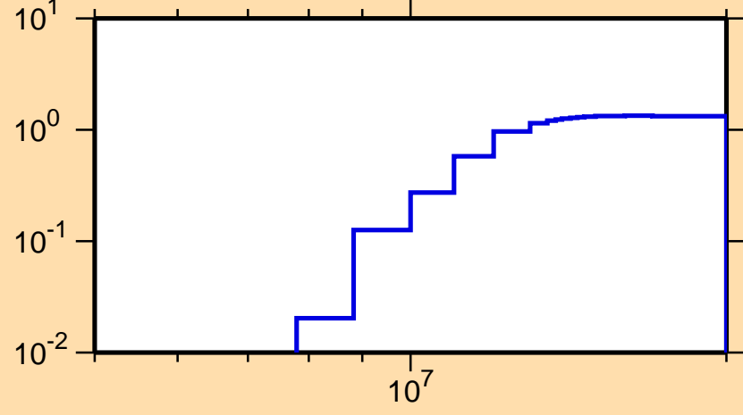
\sigma vs. E for ^{149}\text{Dy}(n,2n)
